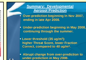
Fig. 7. Regional analysis for 1-h aerosol predictions, Apr 2007 - Aug 2008. The decrease in the Fraction Correct (FC) in Dec 2007 and subsequent increase in May 2008 is associated with a change in the model from over-prediction to under-prediction.
