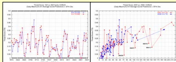
Fig. 8. 8-h ozone, TS for 0600 UTC cycle is slightly better than 1200 UTC in 2008.
