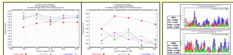
Fig. 6. Regional analysis for 8-h ozone predictions, June 15 – Aug 31, 2008. The Pacific Coast (PC) region shows the highest Threat Score (TS) and lowest mean bias. The TS for the PC region was higher in 2008 than in 2007.
