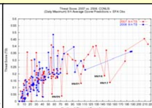
Fig. 9. 8-h ozone, Threat Score vs. number of observed exceedances, 2008 vs. 2007, more under-prediction in June, 2007.
