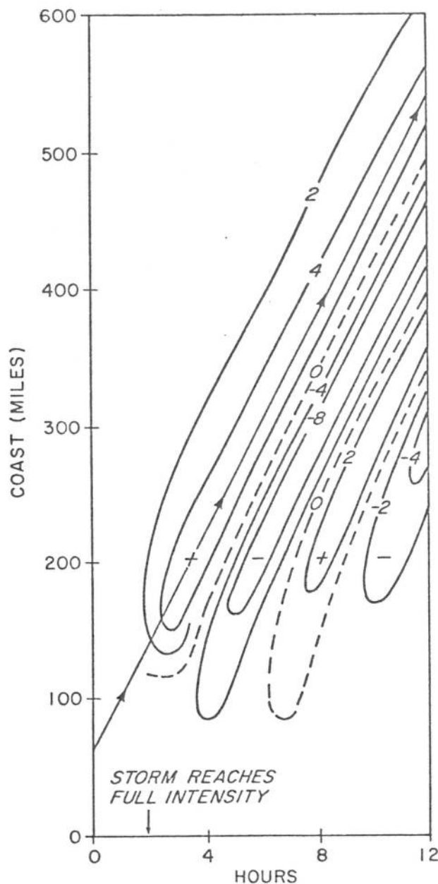
FIGURE 6.—Same as figure 5 for a standard storm, in a standard basin, and traveling parallel to the coast at 40 m.p.h. with center of the storm 40 mi. seaward. This figure shows formation of traveling edge waves on the coast.
