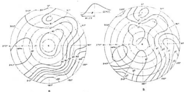
FIGURE 14.—Distance, in statute miles, from peak surge to minimum surge on the coast. Arguments same as figure 7.
