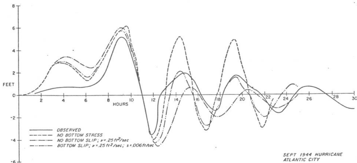
FIGURE 21.—Observed and computed surges, against time, at Atlantic City for the September 1944 storm. The basin used in the computations is given in figure 20. Hours are for model time.
