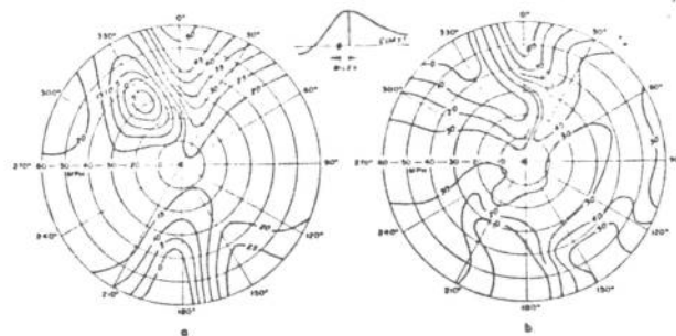
FIGURE 7.—Contours of distance, in statute miles, from landfall position to point of peak surge on the coast. Radii are storm speeds, rays are crossing angles of storm track to the coast (standard storm in standard basin). (a) Radius of maximum wind, 15 statute mi. (b) Radius of maximum wind, 30 statute mi.
