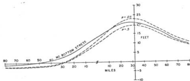
FIGURE 23.—Same as figure 22 with bottom slip s equal to 0.006 ft./sec.
