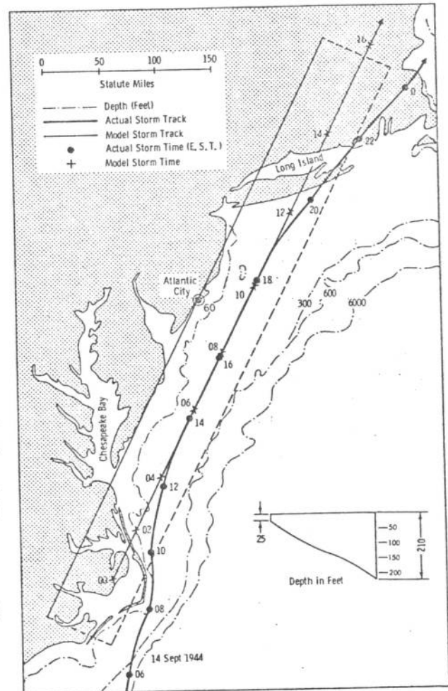
FIGURE 20.—Orienting a model basin along a portion of the Eastern Seaboard of the United States; the depths chosen for the one-dimensional model basin is shown in the insert, and is the mean depths about Atlantic City. The model track, simulating the natural storm track, for the September 1944 hurricane, is shown.
