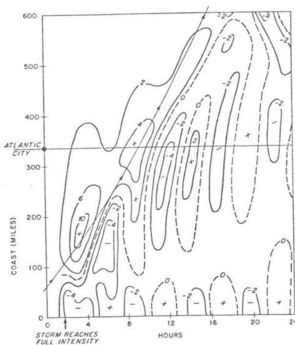
FIGURE 5.—The computed coastal surge profile, contoured against time, for the September 1944 storm modeled in Appendix II. The line with arrows represents the position of the storm center normal to the coast (center of storm 40 mi. seaward). This figure shows the formation of shelf seiches behind the storm's center.
