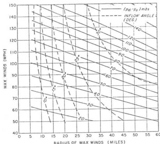
FIGURE 2.—A nomogram relating three model storm parameters, stationary storm maximum wind, radius of maximum wind in statute miles, and pressure drop. The inflow angle occurs 100 mi. from the storm center. The storm center is at latitude 30^\circ .
