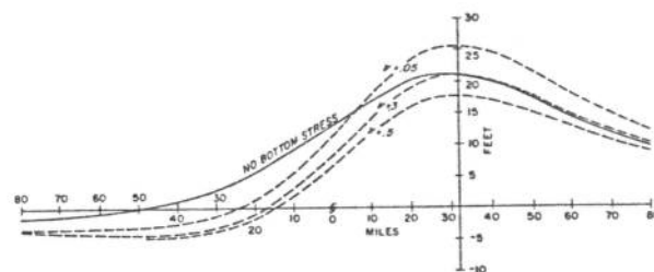
FIGURE 22.—Comparison of computed surge profiles, without and with bottom stress (equation (10)), generated by a fast moving storm traveling normal to the coast. The eddy viscosity coefficient \nu ranges through an order of magnitude; no bottom slip.
