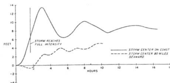
FIGURE 4.—The computed height of the peak surge against time generated by a stationary storm.
