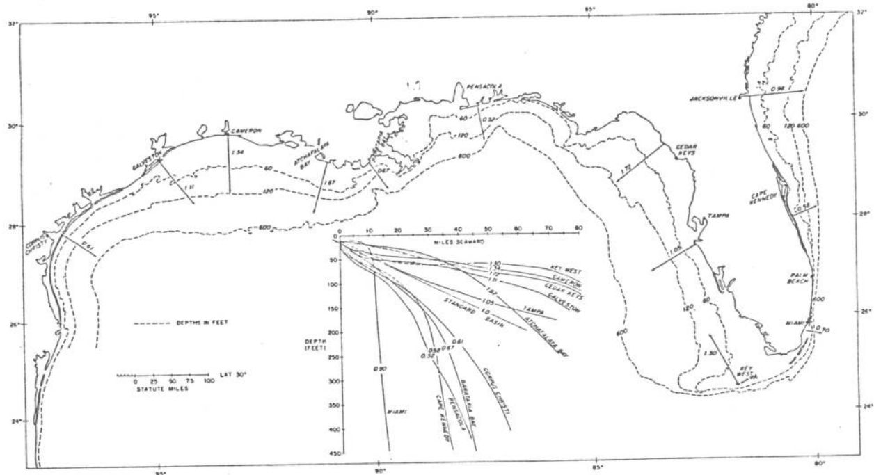
FIGURE 18.—Same as figure 17 for the Gulf States and Florida.
