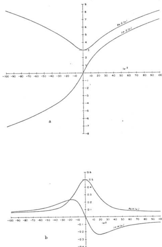
FIGURE 19.—(a) Plot of real and imaginary parts of G(\sigma) against i\sigma^2 . (b) Plot of real and imaginary parts of H(\sigma) against i\sigma^2 .
