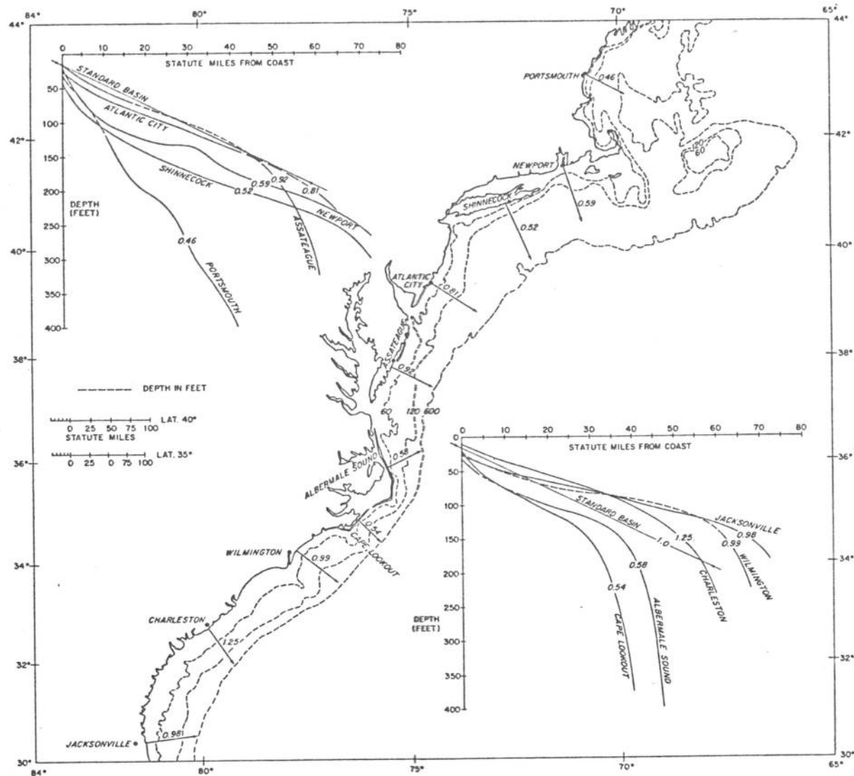
FIGURE 17.—Correction factors at selected points along the Eastern Seaboard of the United States for depth profiles other than standard; the factors are used to correct pre-computed surge heights in a standard basin. The inserts are the mean depth profiles of the selected points.
