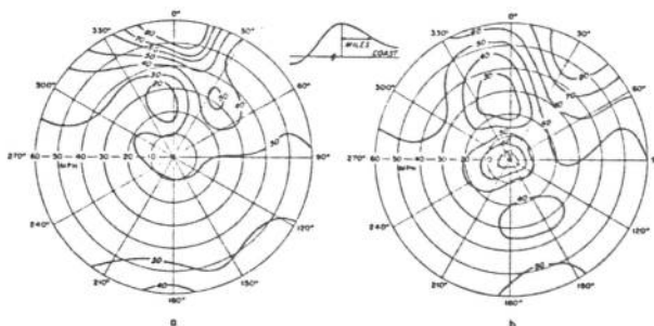
FIGURE 9.—Same as figure 8 for the minimum surge, portrayed at time of the peak surge. The absolute minimum surge does not necessarily occur at time of peak surge.
