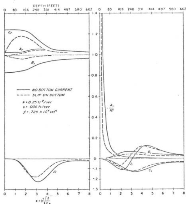
FIGURE 1.—Real and imaginary parts of the four coefficients ( A , B , C , J ) of equations (9) and (17) as functions of Ekman number " e " or depth.
