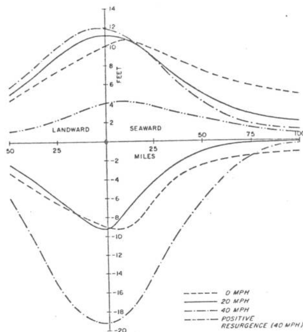
FIGURE 16.—Height nomogram of the directly generated crest and trough, and the resurgence amplitude, for storms (standard storm and standard basin) moving at different speeds parallel to the coast. The abscissa is distance of the storm center from the coast in statute miles.
