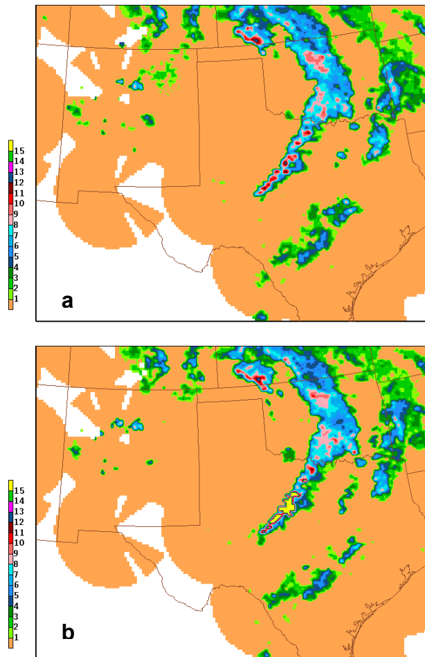
Figure 5. WSI reflectivity for (a) 0200 GMT and (b) 0215 GMT, 23 April 2000. The reflectivity categories are defined in Table 1. The abrupt increase in reflectivity seen in (b) was not associated with a corresponding increase in the CTG lightning rate.
