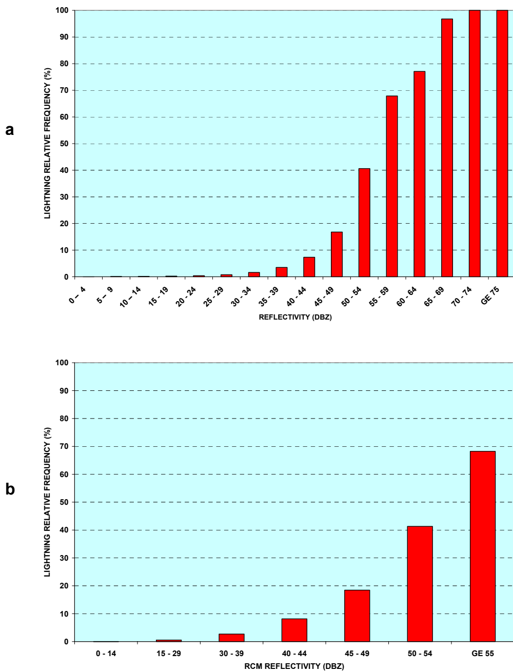
Figure 12. Same as Fig. 2 (a) and Fig. 3 (b) following application of all quality control procedures.
