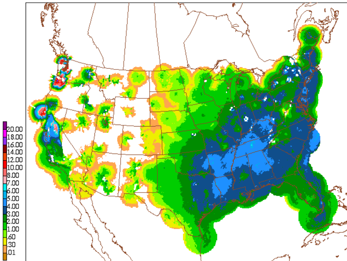
Figure 11. Cool season echo relative frequency (%) for WSI reflectivities of \geq 30 dBZ following application of all QC procedures.
