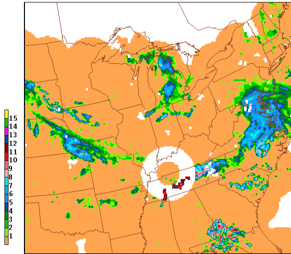
Figure 13 . Same as Fig. 4, except following application of all WSI quality control processes.
