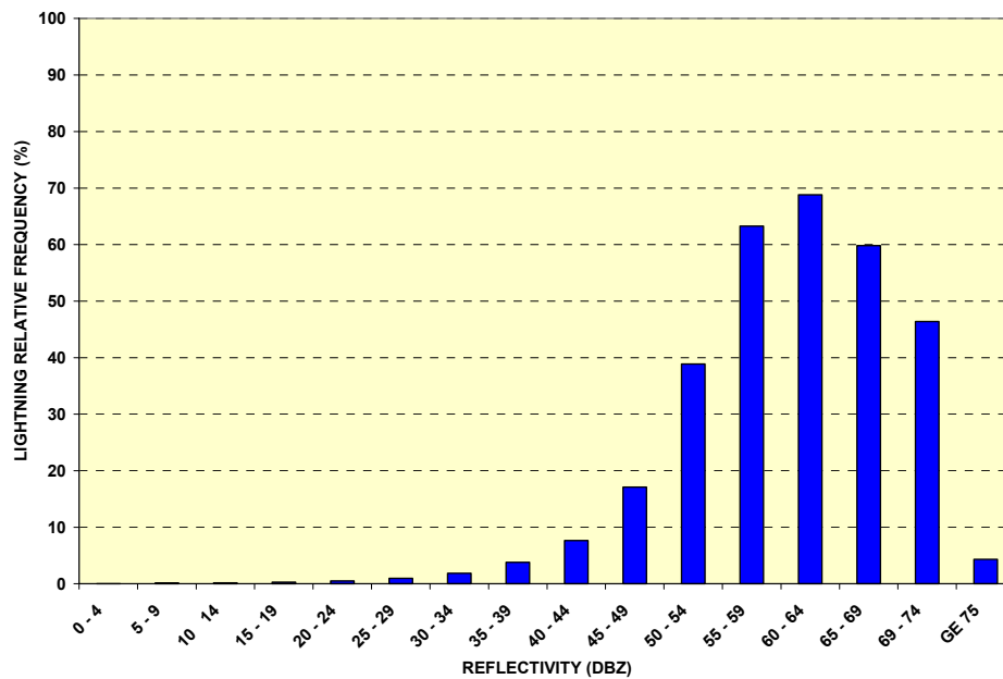
Figure 2. Lightning relative frequency versus WSI reflectivity. The data are from the CONUS, the 1997-2001 warm season (April – September) months, and all clock hours. The radar data have a nominal time of :30 and the lightning reports are valid :20 - :35 (times are minutes past the hour)
