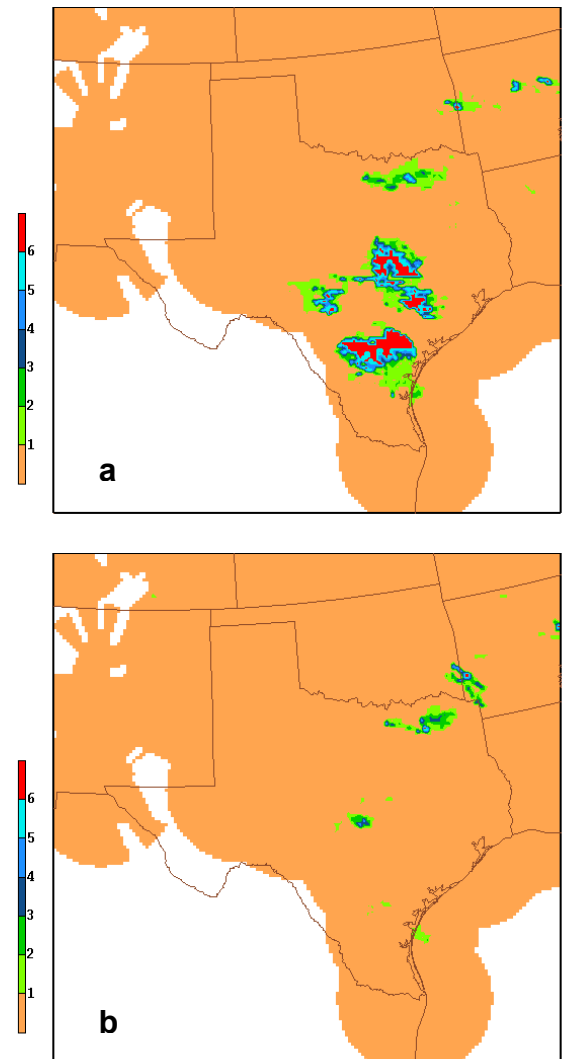
Figure 6. RCM reflectivity for (a) 0715 GMT and (b) 0815 GMT, 30 April 2002. CTG lightning or significant precipitation did not occur at either time. The reflectivity categories are defined in Table 1.
