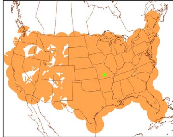
Figure. 1. Composite contiguous US coverage (orange shading) of WSR-88D network radars. The coverage umbrella of each radar is to 230 km, except for locations of substantial terrain occultation in western states. The small green-shaded square in the central US illustrates the size of a 10 x 10 array of the 10-km WSI/RCM gridboxes.
