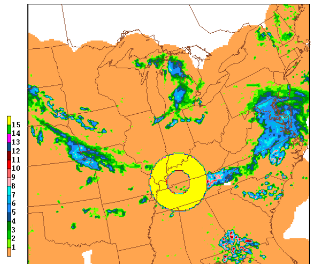
Figure 4. WSI reflectivity for 1845 GMT, 21 April 1997. The reflectivity categories are defined in Table 1. The \geq 75 dBZ test pattern is from the Ft. Campbell, KY WSR-88D site.
