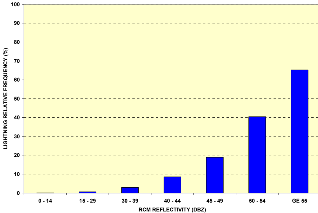
Figure 3. Same as Fig. 2 for RCM reflectivities, the :15 radar nominal time, and the 2002-03 warm seasons.
