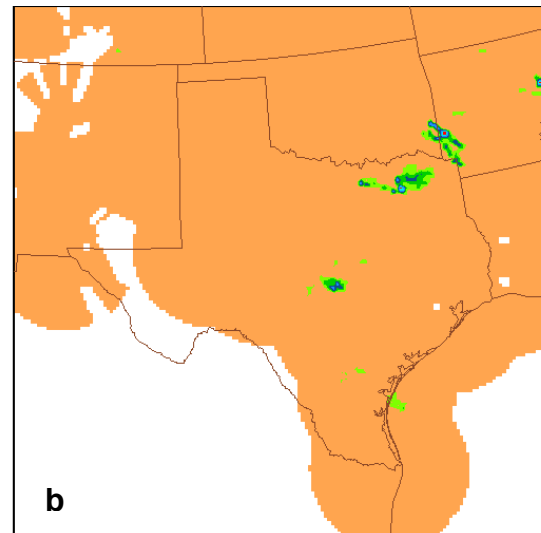
Figure 15. Same as Fig. 6, except following application of all RCM quality control processes.
