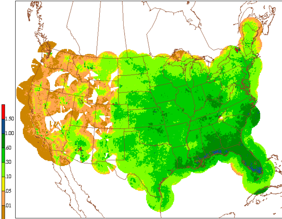
Figure 8. Warm season relative frequency (%) of WSI reflectivities of \geq 50 dBZ after application of the first screening procedure. The sample consists of all :30 radar nominal times and the April – September months of 1997 - 2001. The small red spots depict spurious frequency peaks.
