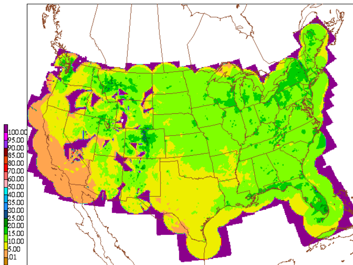
Figure 7. Warm season relative frequency of \geq 5 dBZ WSI reflectivities in 10-km gridboxes. Relative frequencies of 100% appear for gridboxes beyond 230 km to the nearest radar and for gridboxes with substantial radar beam occultation.
