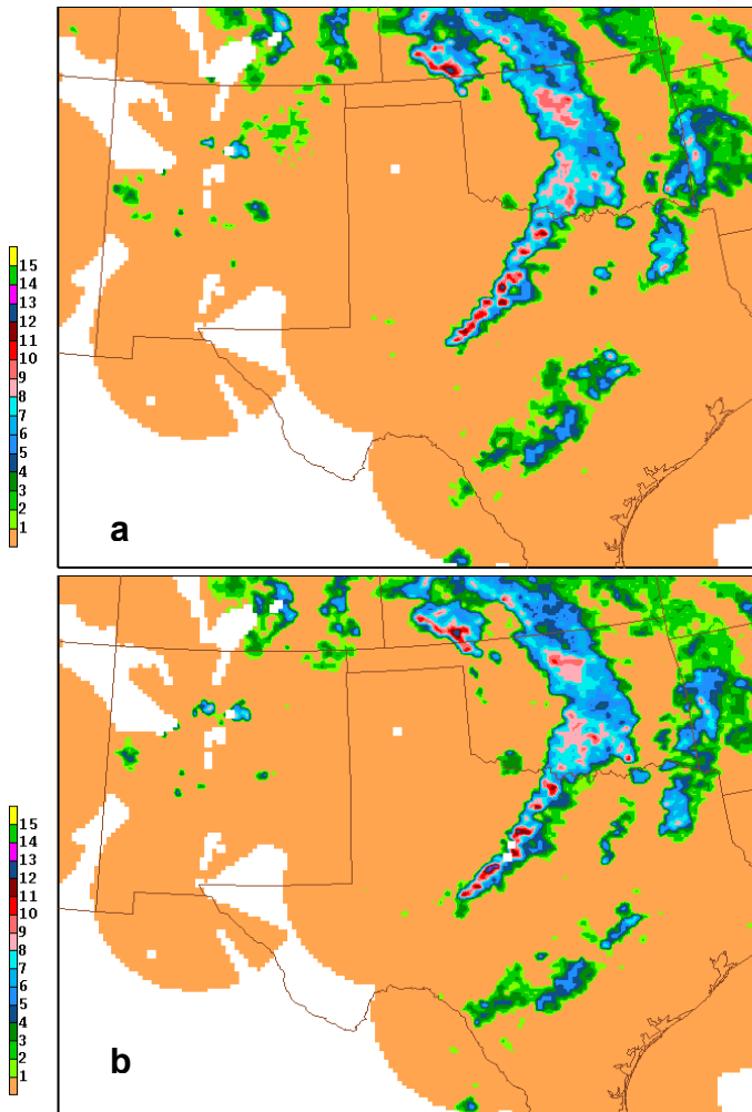
Figure 14. Same as Fig. 5, except following application of all WSI quality control processes.
