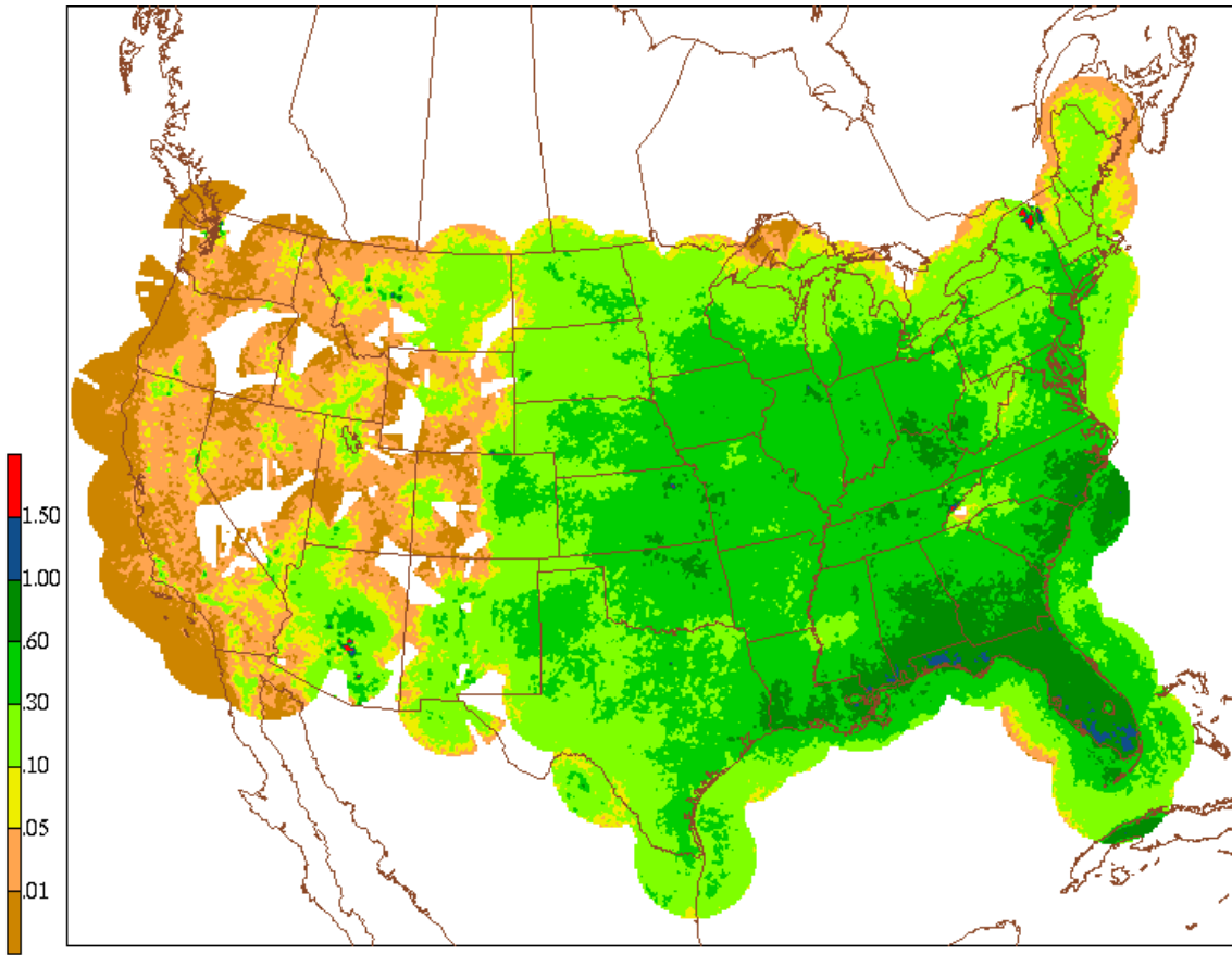
Figure 9. Same as Fig. 8, except with the inclusion of the decision-tree reflectivity checking (second QC procedure).
