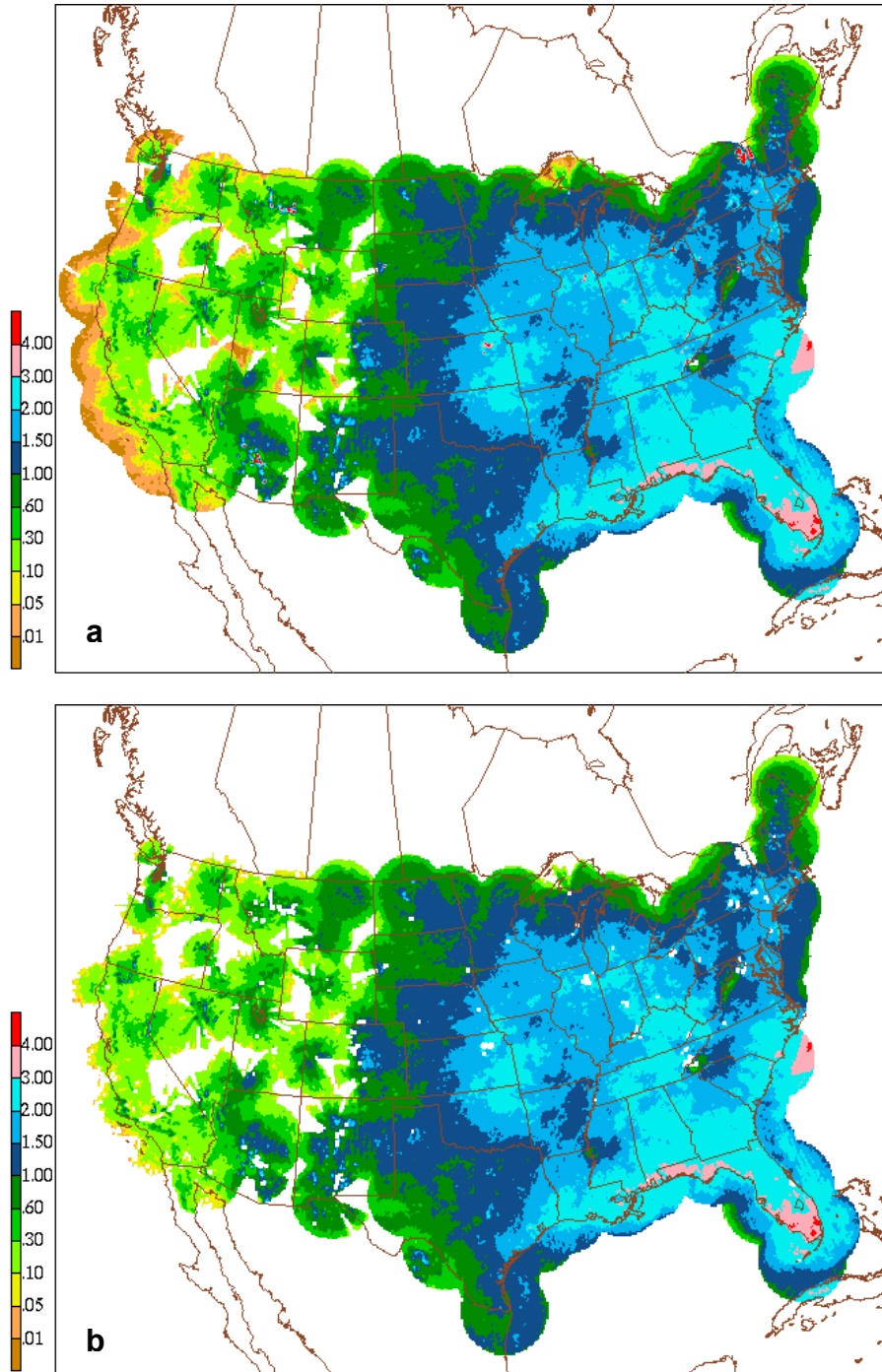
Figure 10. Warm season echo relative frequency (%) for WSI reflectivities of \geq 40 dBZ before (a) and after (b) application of the final screen.
