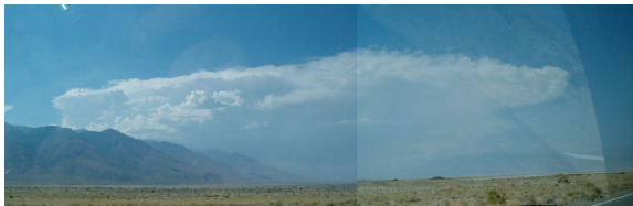
Figure 5 – Panoramic photograph of thunderstorm that spawned Rockwell Pass tornado taken on 07 July between Lone Pine and Keeler, CA, at 2317 UTC (4:17 PM PDT), looking to the northwest. Note the backsheared anvil and overshooting top. (Photo by Bill Hensley)
