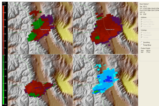
Figure 11. Doppler radar radial velocity at 0.5°, 1.5°, and 2.4° elevation angles, and reflectivity at 0.5° elevation angle from KEYX at 2340 UTC 7 July 2004. Location of the tornado at Rockwell Pass is shown as a red dot.
