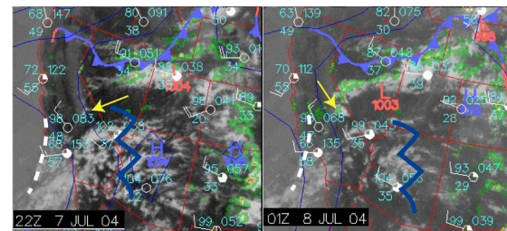
Figure 8 – Fronts and selected surface observations and infrared satellite imagery for selected hours on the day of the Rockwell Pass tornado. White dashed/blue jagged line show the positions of the 300 mb short wave trough and downstream ridge (as explained in the text) at the same times. Yellow arrow shows the position of the Rockwell Pass thunderstorm. (Charts courtesy of Unisys)
