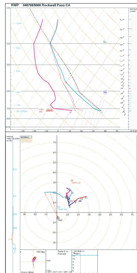
Figure 9. Proximity sounding and hodograph (generated by NSHARP) at 0000 UTC 8 July 2004, as explained in the text.
