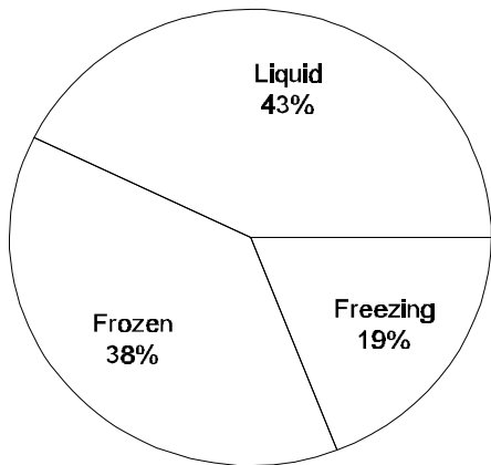
Figure 3. Typical distribution of precipitation states.
