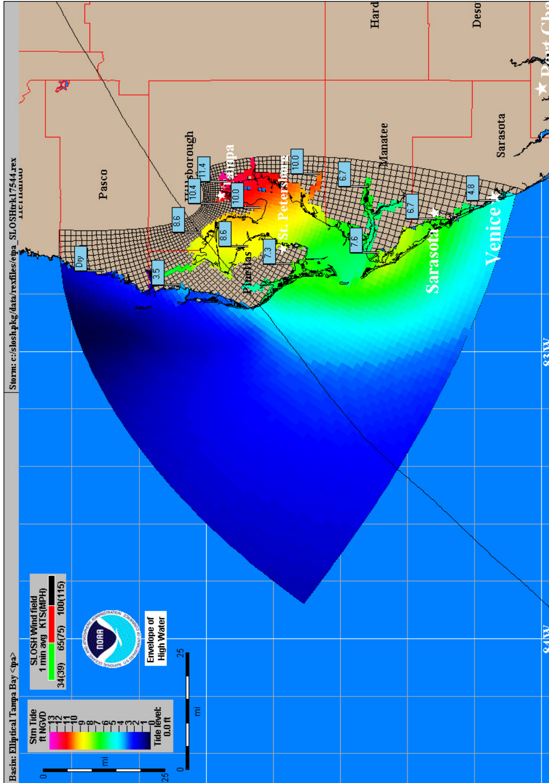
Figure 5. SLOSH Simulation showing Effect of Hurricane Track Number 17544 on the Tampa Bay Basin
