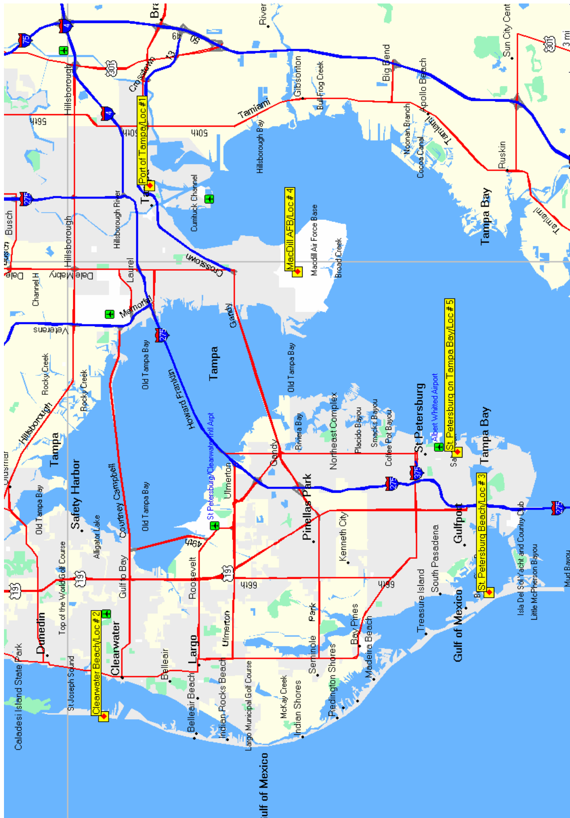
Figure 1. Locations of Five Sites of Interest in the Tampa Bay Basin
