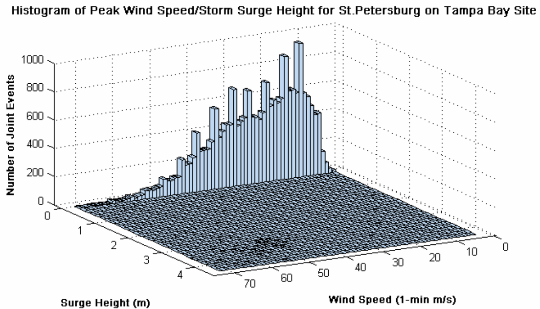
Figure 6(e) Joint Histogram of Peak Wind Speed/Surge Height for St. Petersburg on Tampa Bay
