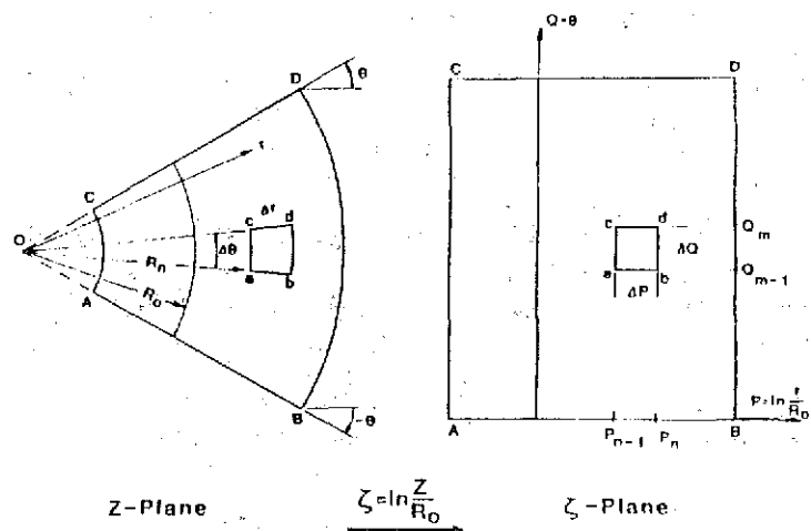
Figure 1. Transforming an (R,θ), unequally spaced polar grid in the Z-Plane onto an (P,Q), equally spaced, rectangular grid in the \zeta -Plane.
