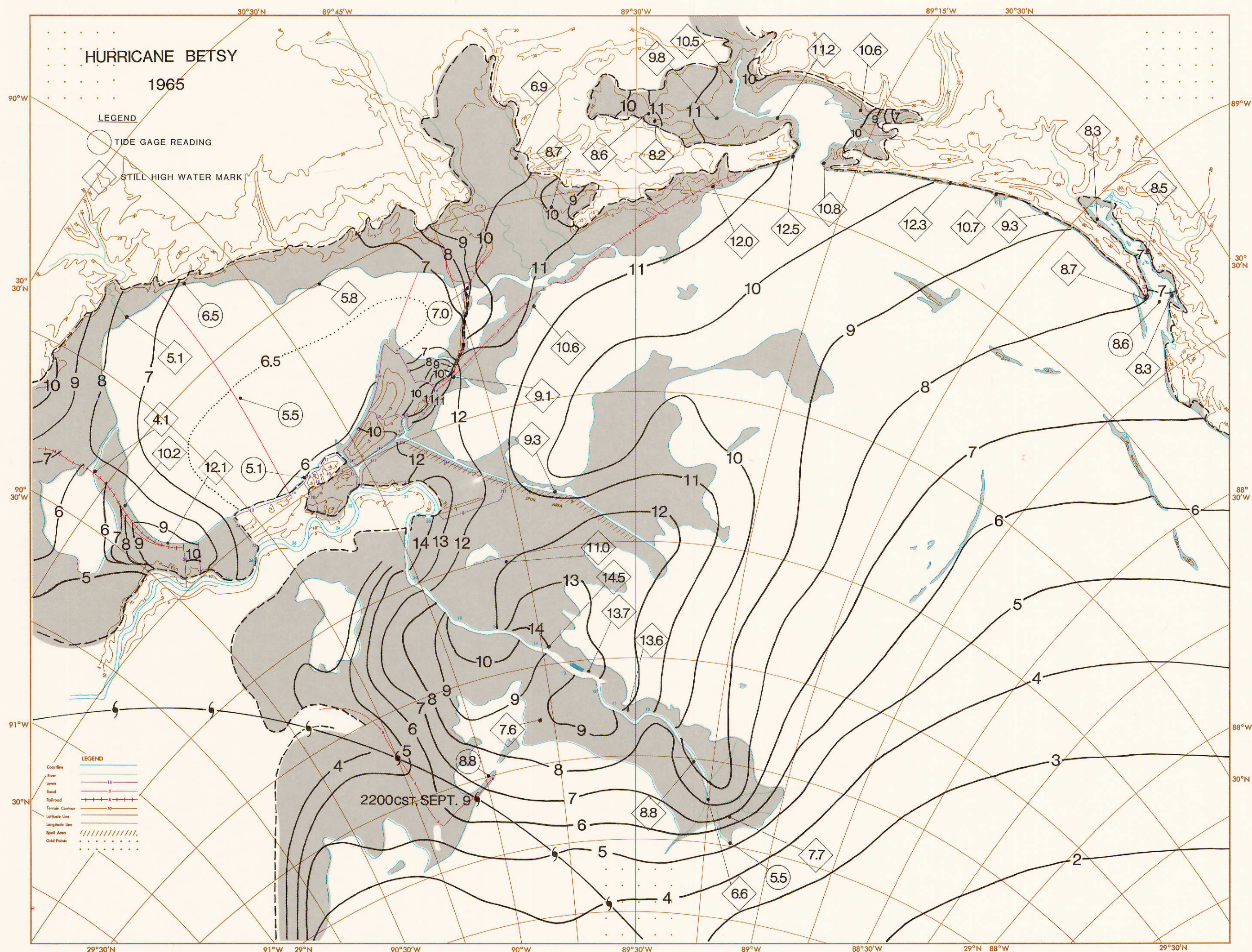
Figure 22. Contoured surface envelope of highest computed surges for Hurricane Betsy, 1965 and the extent of inundation. The contours are hand drawn from Fig. 19 with the overlay, Fig. 20, placed over it. The contours begin and terminate when the surge height reaches the local terrain height. The Shaded area indicates inundation over land. Observed surge heights are also shown for comparison to computed values. Tide and river gage maximum surges are shown within circles; high water mark heights are shown within diamonds.
