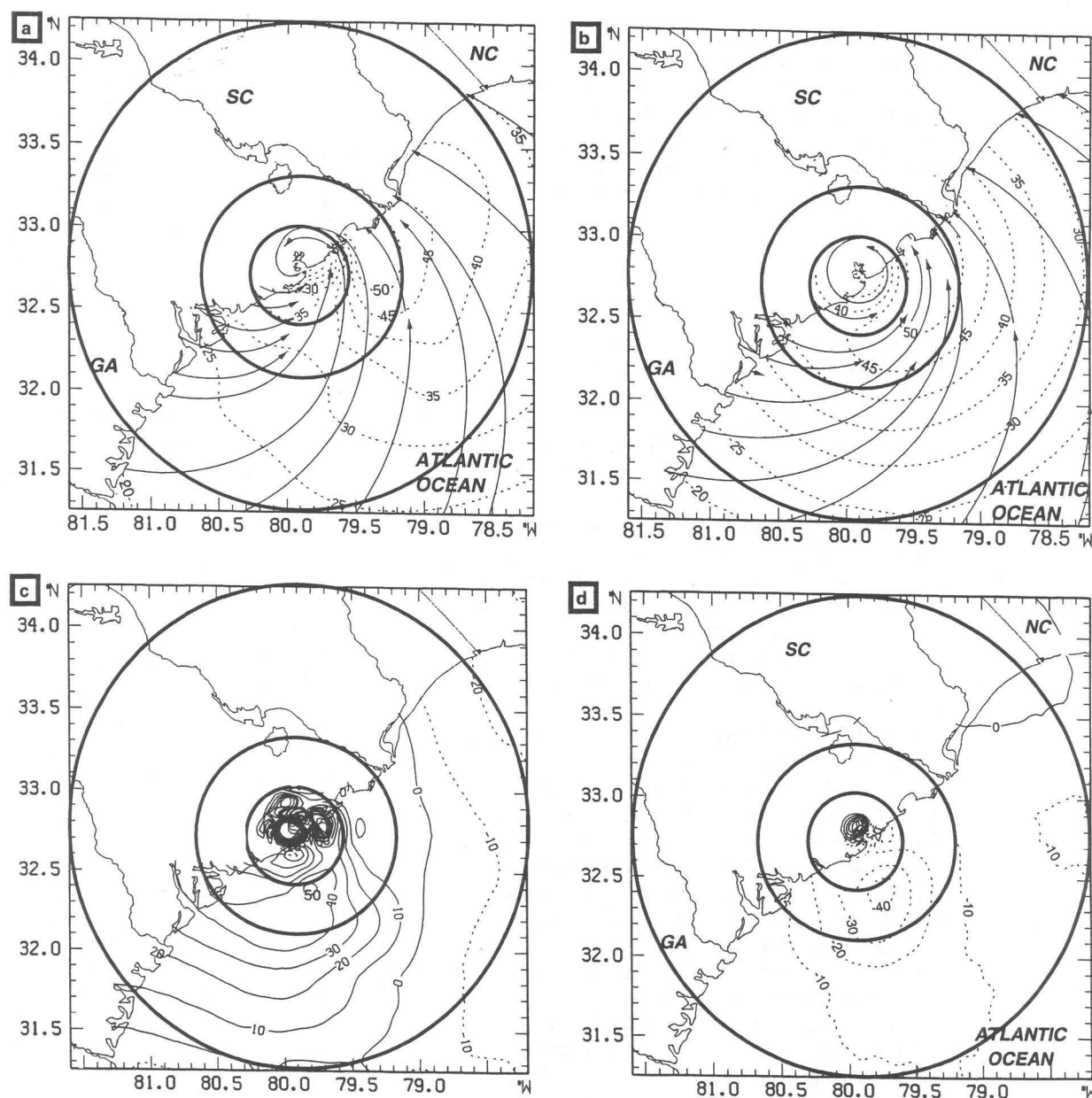
FIG. 2. Wind fields over water for Hurricane Hugo at 0405 UTC 22 Sep 1989. The winds are displayed as streamline and isotachs (units of wind speed are \text{m s}^{-1} ). The range rings are 0.75R_{\text{MW}} (inner), 1.50R_{\text{MW}} (middle), and 158 \text{ km} (outer) from the storm center. The winds in (a) are the V_{\text{HRD}} and the winds in (b) are the V_{\text{SLOSH}} . The difference fields are (c) the NWSD field (%) and (d) the IAD ( ^{\circ} ) where dashed contours are negative.
