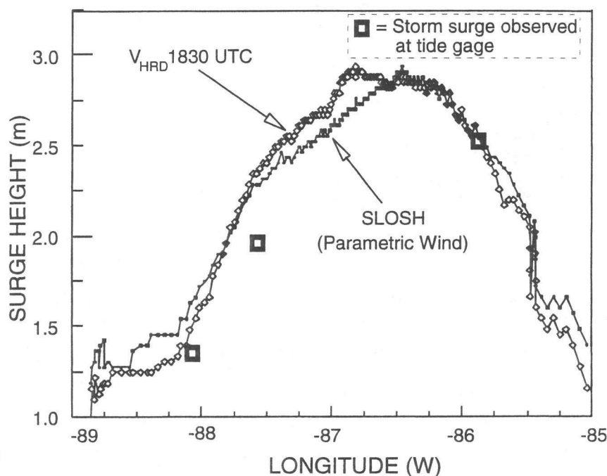
FIG. 6. Hurricane Opal's computed peak storm surges along the Gulf Coast between 85^\circ and 89^\circ W longitude using the V_{SLOSH} and V_{HRD} (1830 UTC) winds as input. The observed peak storm surges from tide gauges (large open squares) in the area of Opal's landfall are shown.
