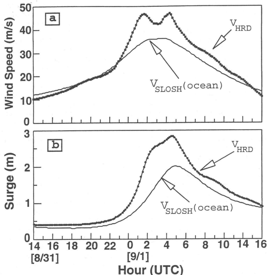
FIG. 7. Time series of (a) Hurricane Emily's V_{SLOSH} (ocean) and V_{HRD} (2200 UTC) and storm surge from 1400 UTC 31 Aug to 1600 UTC 1 Sep 1993 wind speeds ( \text{m s}^{-1} ) and (b) computed peak storm surge values on the Pamlico Sound side of Cape Hatteras, NC.
