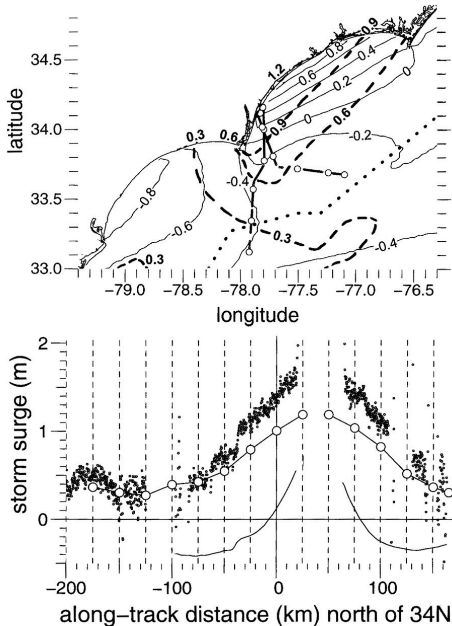
FIG. 10. (top) Circles are spaced at 25-km intervals along the aircraft track (except for the last one) relative to the aircraft first reaching 34^{\circ}\text{N} flying north at 2016 UTC. The thin lines indicate the NCSU storm surge contours at 2016 UTC. The thick dashed lines indicate the SLOSH storm surge contours at 2020 UTC. Dots indicate a piecewise linear approximation of the western edge of the Gulf Stream. (bottom) Dots indicate SRA storm surge values along the flight track. The curve without the circles indicates NCSU surge values along the flight track. SLOSH surge values are indicated by the circles connected by line segments.
