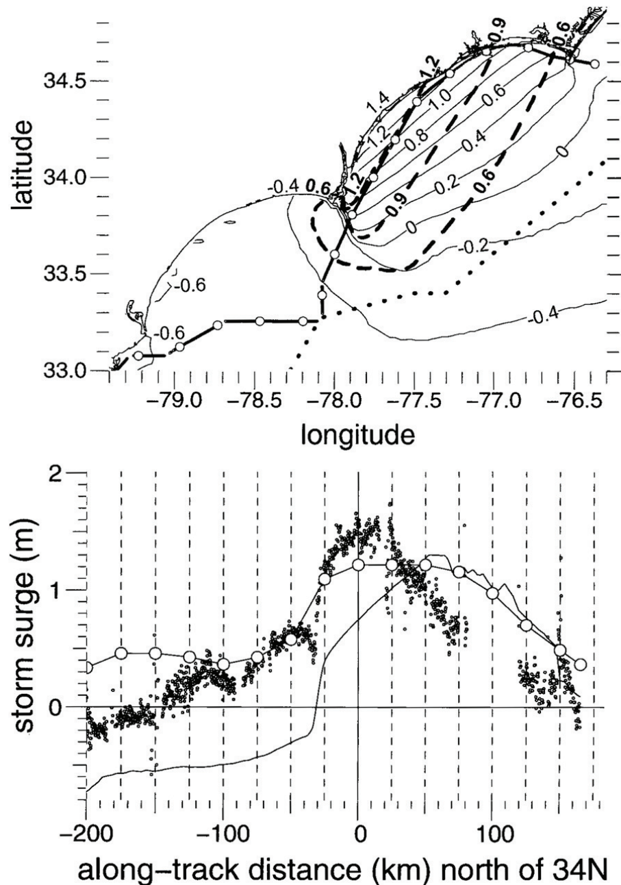
FIG. 9. (top) Circles identify positions along the aircraft track spaced at 25-km intervals (except for the first point) relative to passing 34^{\circ}\text{N} . The thin lines indicate the NCSU storm surge contours at 1828 UTC, when the aircraft passed through 34^{\circ}\text{N} . The thick dashed lines indicate the SLOSH storm surge contours at 1820 UTC. Dots indicate a piecewise linear approximation of the western edge of the Gulf Stream. (bottom) Dots indicate SRA storm surge values along the flight track. The curve without the circles indicates the NCSU surge values along the flight track. SLOSH surge values are indicated by the circles connected by straight line segments.
