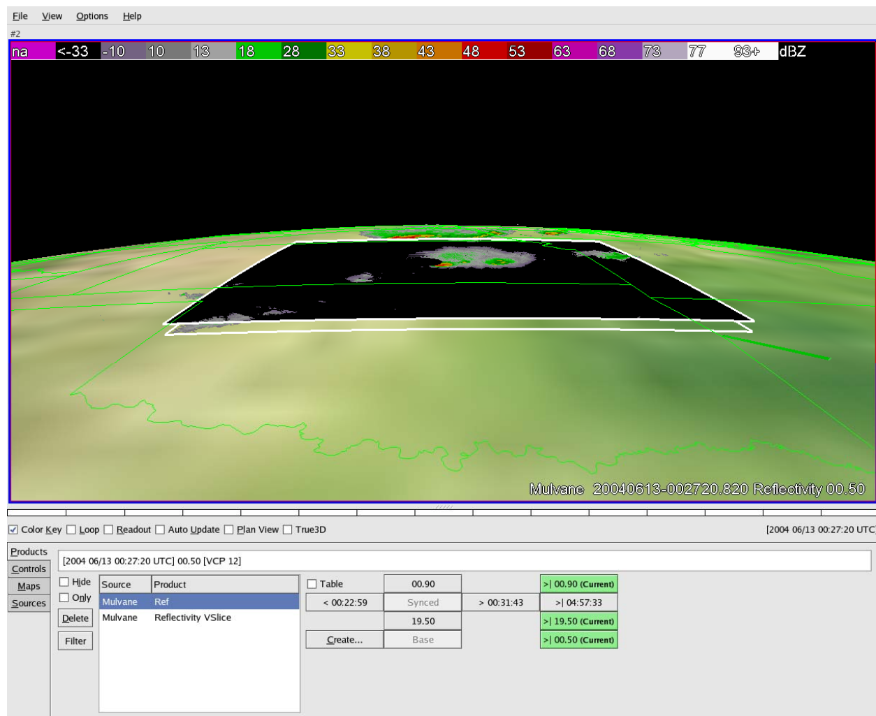
Figure 6: Three-dimensional representation of a horizontal cross-section (CAPPI), drawn large enough to depict a horizontal plane that wraps the Earth's surface in an arced fashion, such that the data on the surface is at a constant altitude above sea-level at all points on the CAPPI surface. Data are from the KICT WSR-88D on 12 June 2004.
