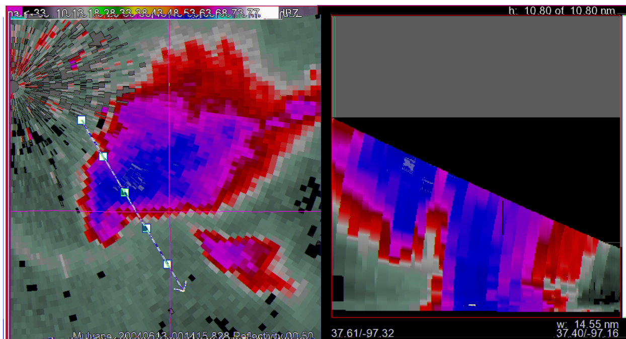
Figure 2: On the left, a constant elevation angle texture (or “PPI display”), and on the right, a vertical cross-section from a classic supercell near Mulvane Kansas on 12 June 2004. Data above the diagonal line on the vertical cross-section are missing due to the radar “cone-of-silence”. Data are from the KICT WSR-88D.
