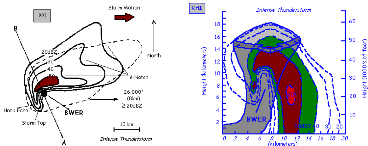
Figure 1: Illustrations of the “Lemon Technique” for operationally identifying supercell thunderstorms using conventional radar (Lemon 1977). On the left is the depiction of a supercell storm using a “Plan Position Indicator” (PPI) display, which is a quasi-horizontal cross-section through the storm (at constant elevation angle). On the right is the depiction of the storm using a “Range Height Indicator” (RHI) display, which is a vertical cross-section, defined by the line A – B on the left image. Various supercell storm features are labeled, including the Bounded Weak Echo Region (BWER).
