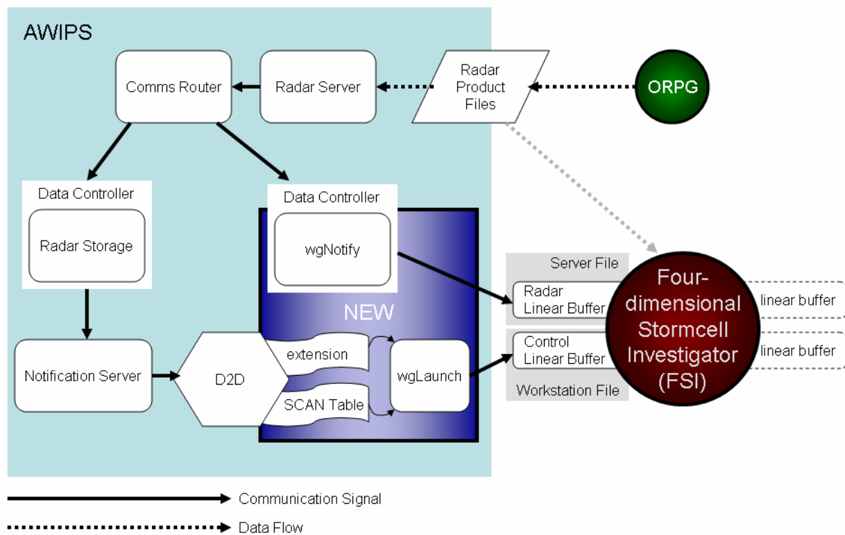
Figure 9: Flow of information and data between the Open Radar Products Generator (ORPG), the Advanced Weather Interactive Processing System (AWIPS), and the Four-Dimensional Stormcell Investigator (FSI).
