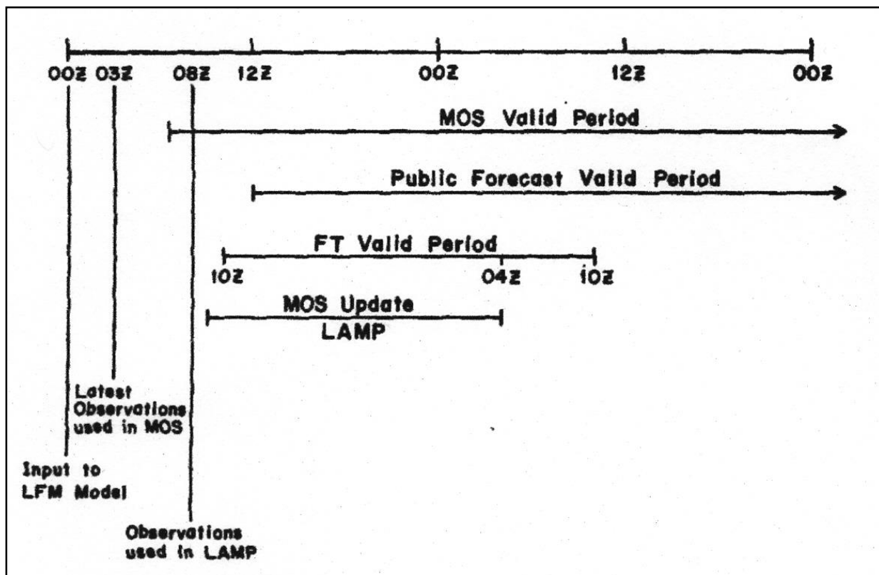
Fig. 18. Relationships among the public and FT (aviation) valid times, the period covered by the LFM-based MOS guidance, and the period for the MOS update system (LAMP). Times are related to the 0000 UTC run of the LFM and the early morning (approximately 0940 UTC) forecast release times existing in 1986.
