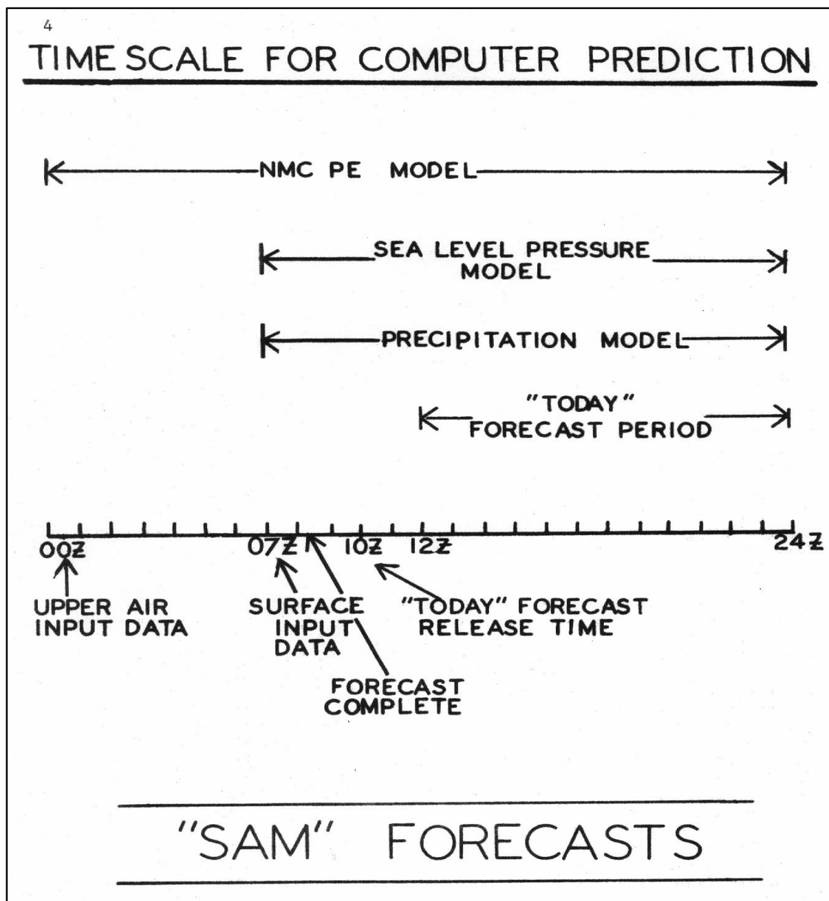
Fig. 1. Temporal relationships among input data, SAM and PE model run times, and the "today" forecast period.
