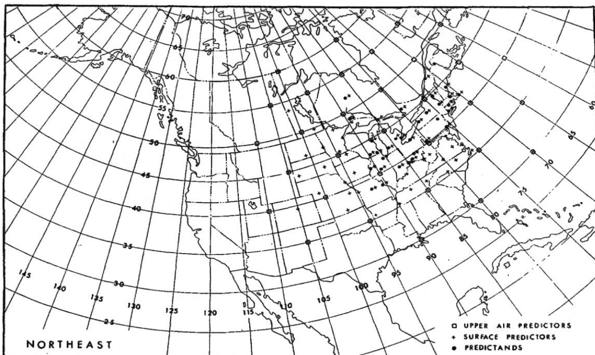
Fig. 8. Network used in development of perfect prog equations for stations in the northeastern U.S.
