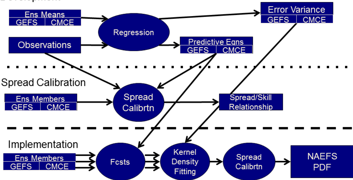
Fig. 2. Graphic depiction of EKDMOS technique
