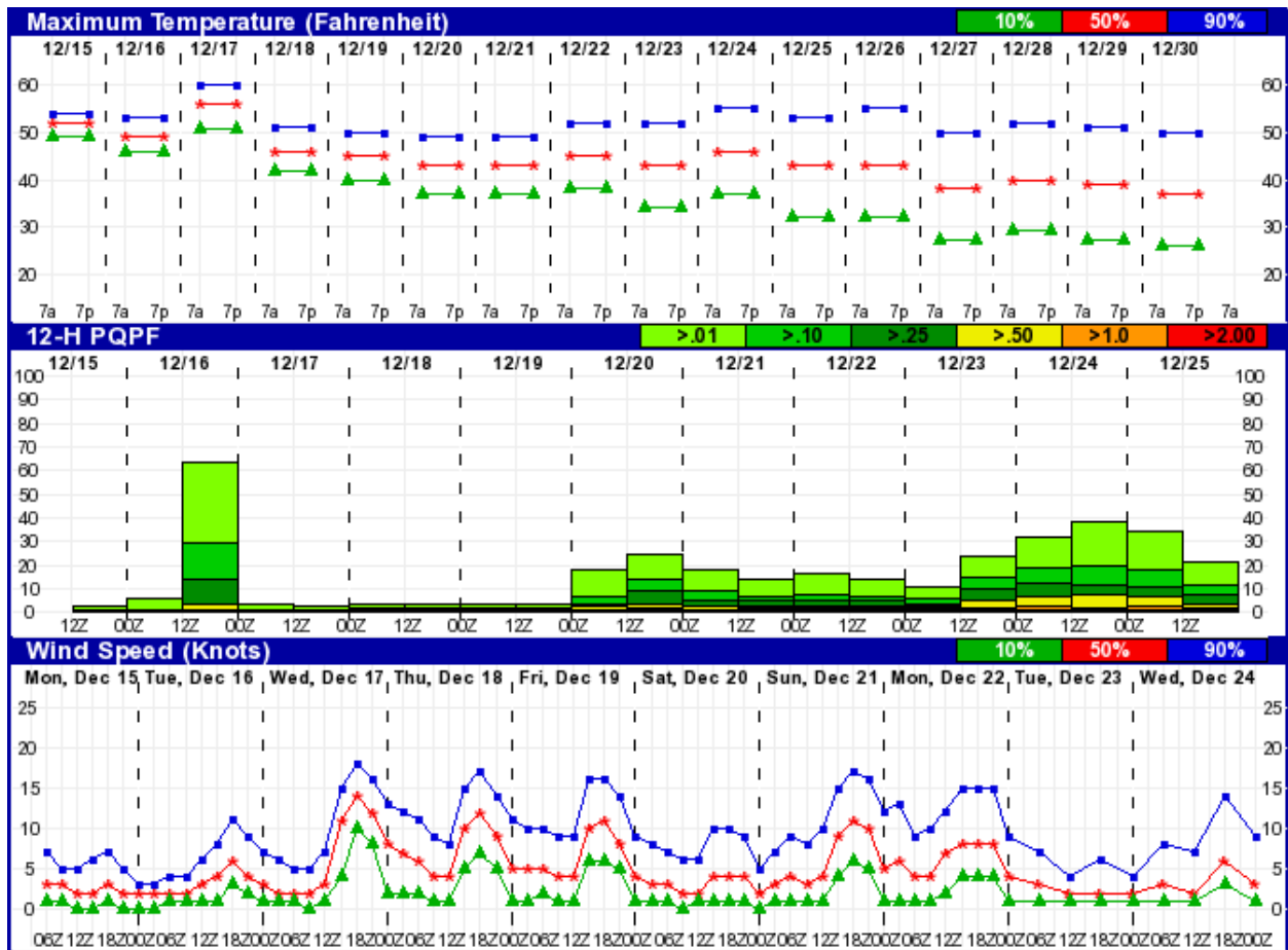
Fig. 5. Sample probabilistic forecasts for daytime maximum temperature, 12-h probabilistic quantitative precipitation forecast, and wind speed visualized as a mixture of 2 meteograms and a stacked histogram.
