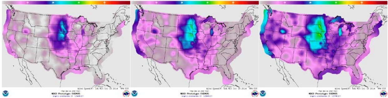
Fig. 4. An example of a gridded probability forecast. These 3 images can be presented as an animation loop. The images depict the 10 th (left), 50 th (middle), and 90 th (right) percentiles of the forecast distribution.
