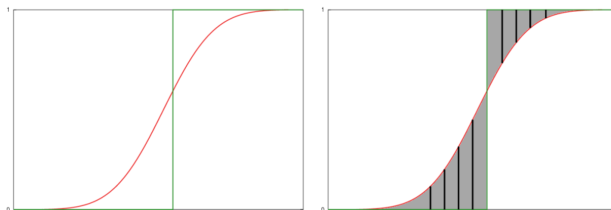
Fig. 8. An illustration of the computation of Continuous Rank Probability Score for a single forecast case. The red curve is the forecast CDF. The green line is a unit step function located at the value of the verifying observation.
