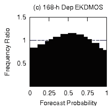
Fig. 7. Sample Probability Integral Transform (PIT) histogram
