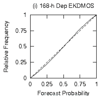
Fig. 6. Sample Cumulative Reliability Diagram
