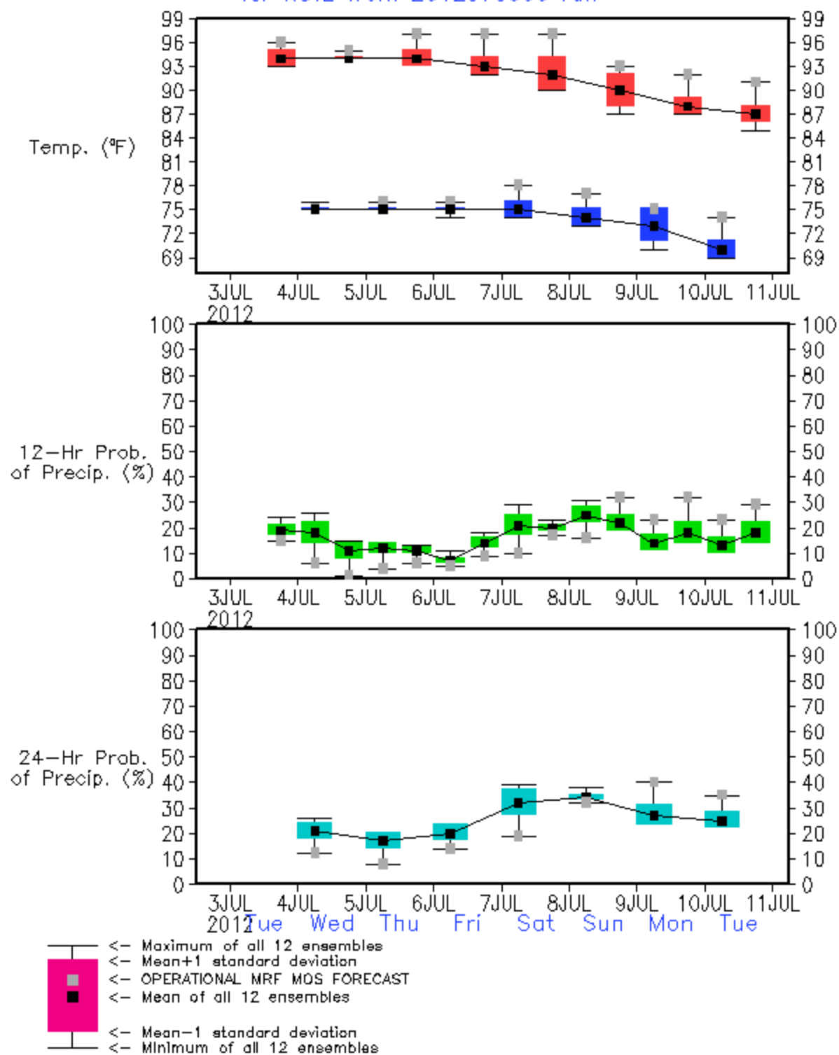
Fig. 1. Sample visualization of a MOS forecast generated from EFS
