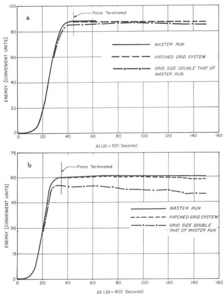
FIGURE 3.—Energy, in convenient units, with time for basins of figure 2 during and after application of a forcing function. (a) Curves for larger basin ( L=470 mi.), (b) Curves for smaller basin ( L=430 mi.).
