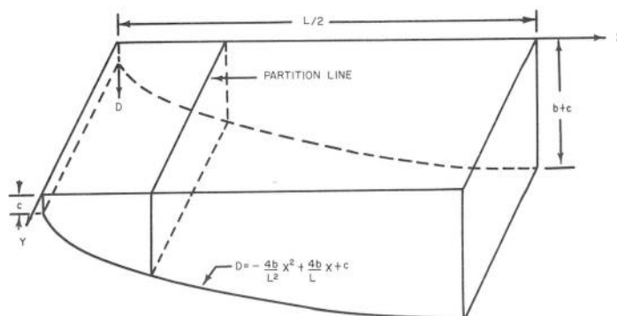
FIGURE 2.—A one-dimensional parabolic depth basin. If two regions of differing grid sizes are used, the partition line patches the regions together.
