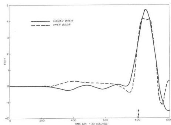
FIGURE 14.—Comparison of height values with time at the point of the shore crossed by the storm.
