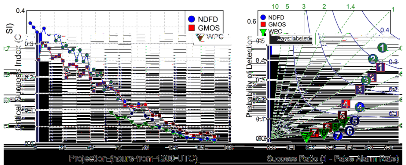
Figure 6. Verification scores for 1200 UTC NDFD, 0000 UTC GMOS, and 0000 UTC WPC freezing/frozen weather type.
