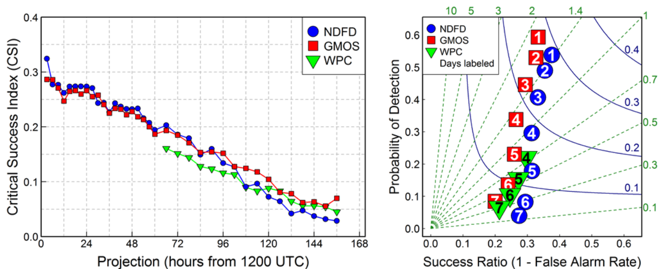
Figure 4. Verification scores for 1200 UTC NDFD, 0000 UTC GMOS, and 0000 UTC WPC liquid weather type.
