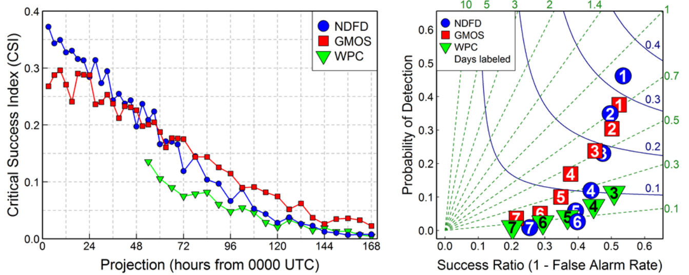
Figure 5. Verification scores for 0000 UTC NDFD, 1200 UTC GMOS, and 1200 UTC WPC freezing/frozen weather type.
