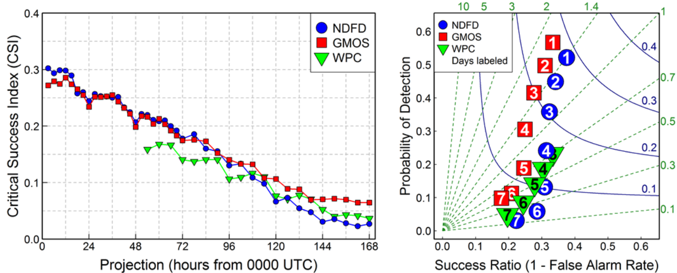
Figure 3. Verification scores for 0000 UTC NDFD, 1200 UTC GMOS, and 1200 UTC WPC liquid weather type.
