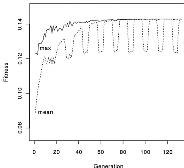
FIG. 4. The GA iteratively tries different weights to improve the fitness. The solid line shows the fitness of the best member at each generation while the dotted line shows the means of the fitness values at each generation as training progresses. The sawtoothed nature of the graph is a result of the periodic use of simulated annealing to perform a local search around each member.
