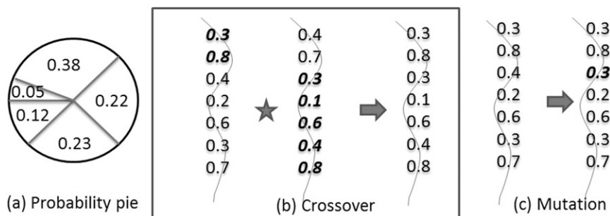
FIG. 1. (a) In a genetic algorithm, chromosomes are chosen probabilistically with better-fit chromosomes more likely to be chosen. The numbers represent the fitness of the chromosome corresponding to the slice. (b) Crossover involves creating a new chromosome that contains the first part of the chromosome of one parent and the second part of the chromosome from another parent. The split point is chosen randomly. The numbers here represent the parameters being tuned (in our case, the weights of each of the interest fields). (c) Mutation involves creating a new chromosome by modifying one of the genes of a parent chromosome.
