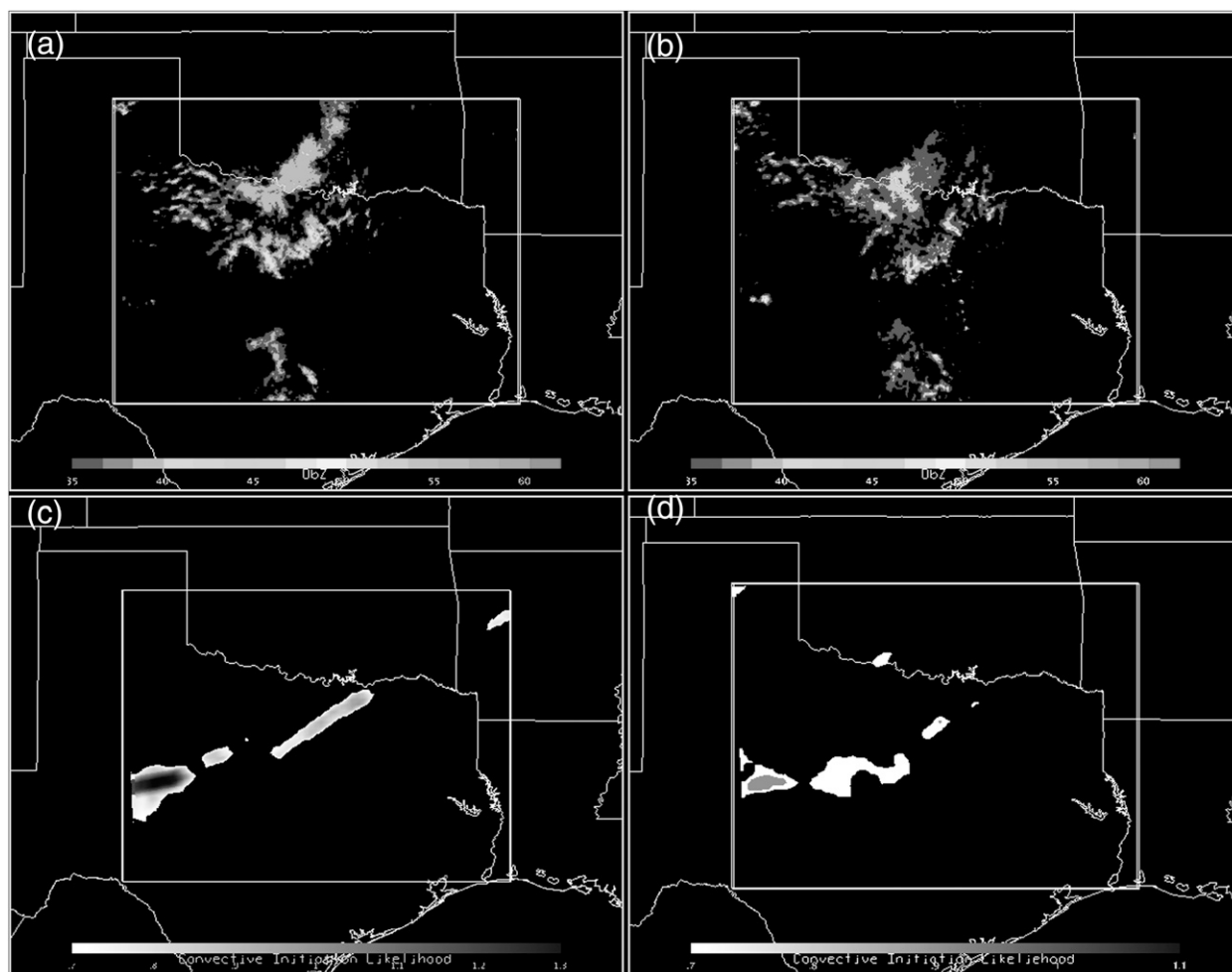
FIG. 2. (a) Radar observation at 1715 UTC 14 May 2010. The domain is centered on the DFW WSR-88D (KFWS) and (b) the radar observation 1 h later. (c) The 60-min initiation nowcast at 1715 UTC by manually tuned ANC and (d) the 60-min initiation nowcast at 1715 UTC by autotuned ANC.
