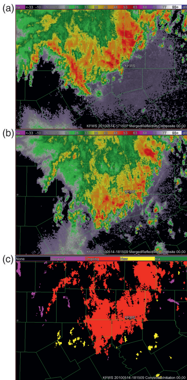
FIG. 3. (a) Radar observation at 1715 UTC 14 May 2010 (detail from Fig. 2a; the location of the radar is marked as KFWS). (b) Radar observation 1 h later. (c) Verification field created by warping the image at 1715 UTC and looking for new convection. The purple shades show decayed convection, reds are ongoing convection, and yellow is new convection.
