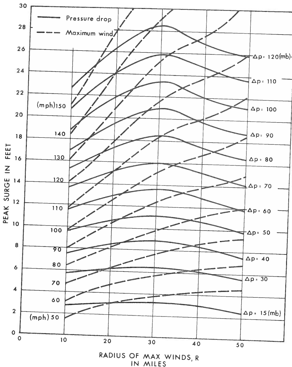
Figure 2. A nomogram of peak surge on the open coast as a function of pressure drop and radius of maximum wind. A standard basin (72 miles wide), standard vector storm motion, and model wind profile were used to form the nomogram. For reference, the maximum wind of the model storm (see fig. A1) is also displayed.
