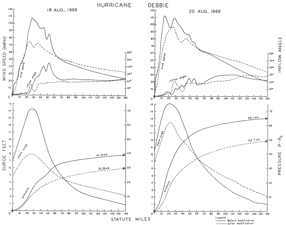
Figure 3. Profiles of observed wind speed and computed inflow angle, pressure, and open coast surge for Hurricane Debbie (1969) before and after storm modifications. The surge is the envelope of high water on the coast for all times. The numbers on the pressure profiles are pressure drop in millibars.
