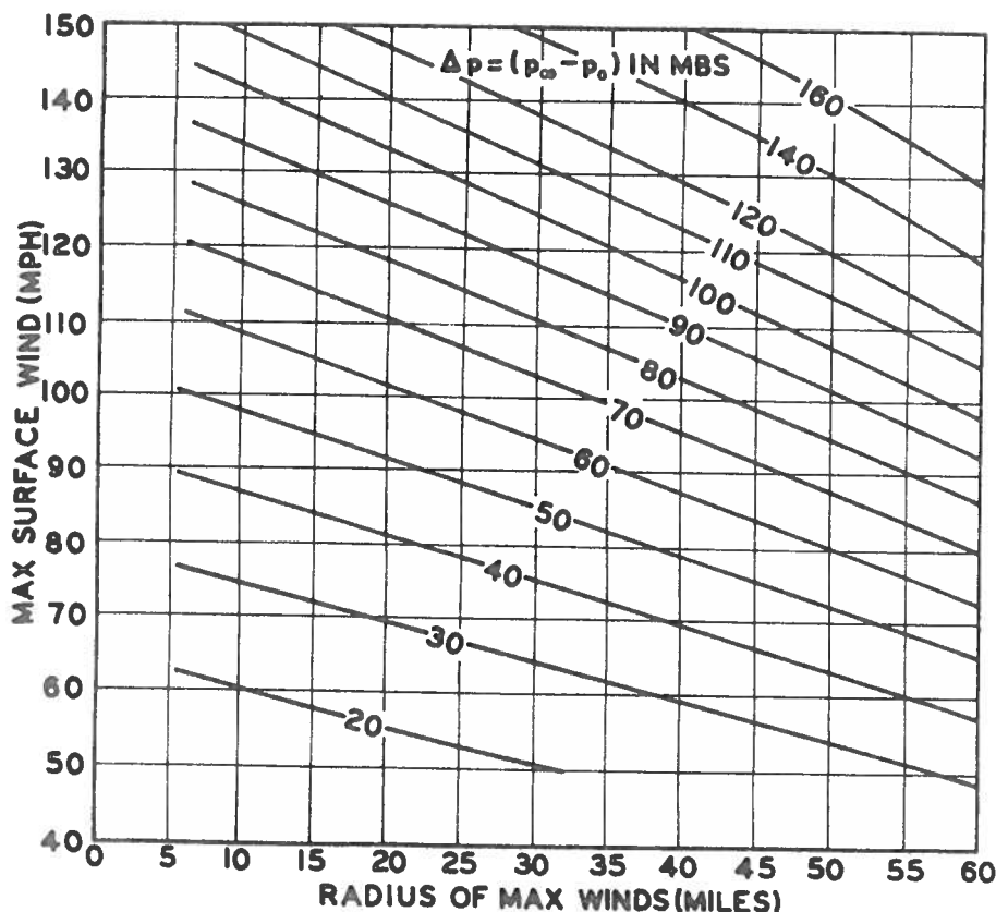
Figure A1. A nomogram relating three storm parameters for a stationary storm; the maximum wind W_M , the radius of maximum wind R , and the pressure drop of the storm \Delta P . The storm center is at latitude 30^\circ .
