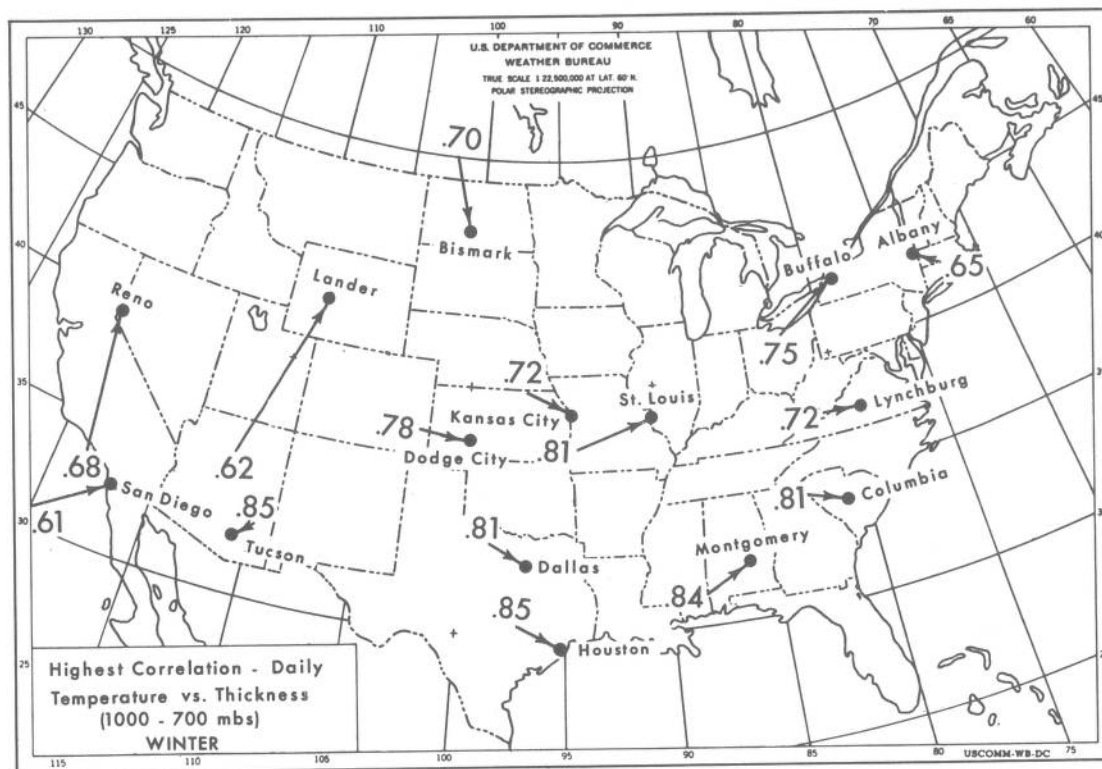
Figure 13. - Center and magnitude of maximum correlation between anomalies of mean daily temperature at the cities indicated and 700-1000-mb. thickness on the same day for 140 winter cases.
