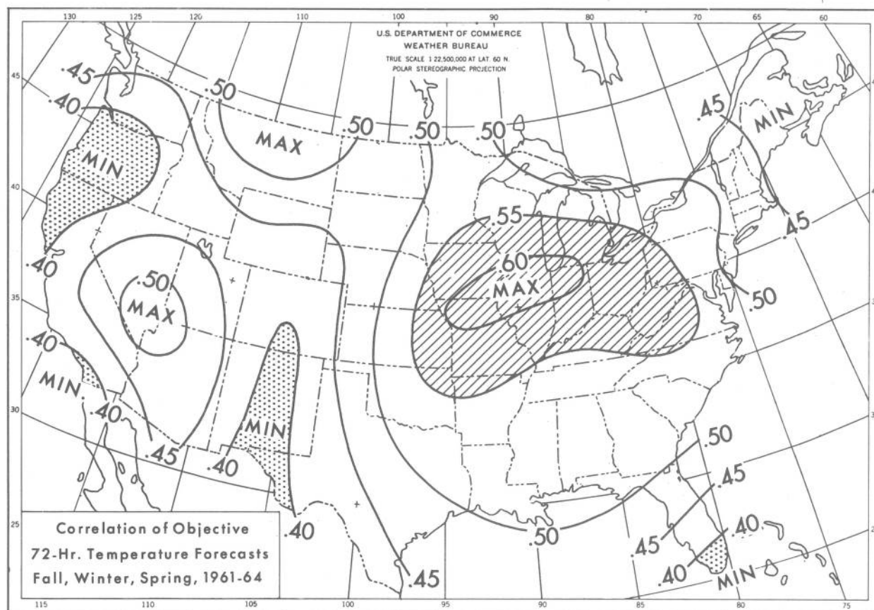
Figure 2. - Simple linear correlation coefficients between standardized anomalies of objective 72-hr. temperature forecasts and verifying temperatures during fall, winter, and spring seasons from 1961 to 1964, with centers labeled as maximum or minimum.
