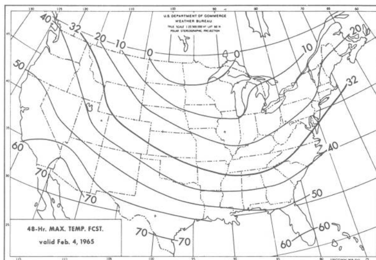
Figure 4. - A sample 48-hr. maximum temperature forecast transmitted over facsimile by the National Meteorological Center on February 2, 1965. Isotherms are labeled in °F.
