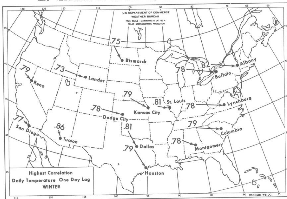
Figure 14. - Center and magnitude of maximum correlation between anomalies of mean daily temperature at the cities indicated and mean daily temperature on the previous day for 140 winter cases.
