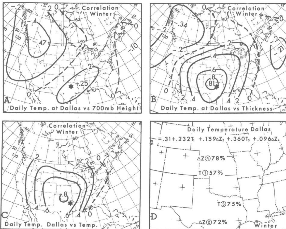
Figure 11. - Correlation fields between anomalies of mean daily temperature at Dallas, Tex. (located by the star) for 140 winter cases and (A) 700-mb. height on the same day; (B) 700-1000-mb. thickness on the same day; (C) mean daily temperature on the previous day. Part D illustrates the multiple regression equation derived by screening. T is the temperature anomaly in ^{\circ}\text{F} , \Delta Z is the thickness anomaly in tens of feet, and the explained variance after inclusion of each variable is given in percent.
