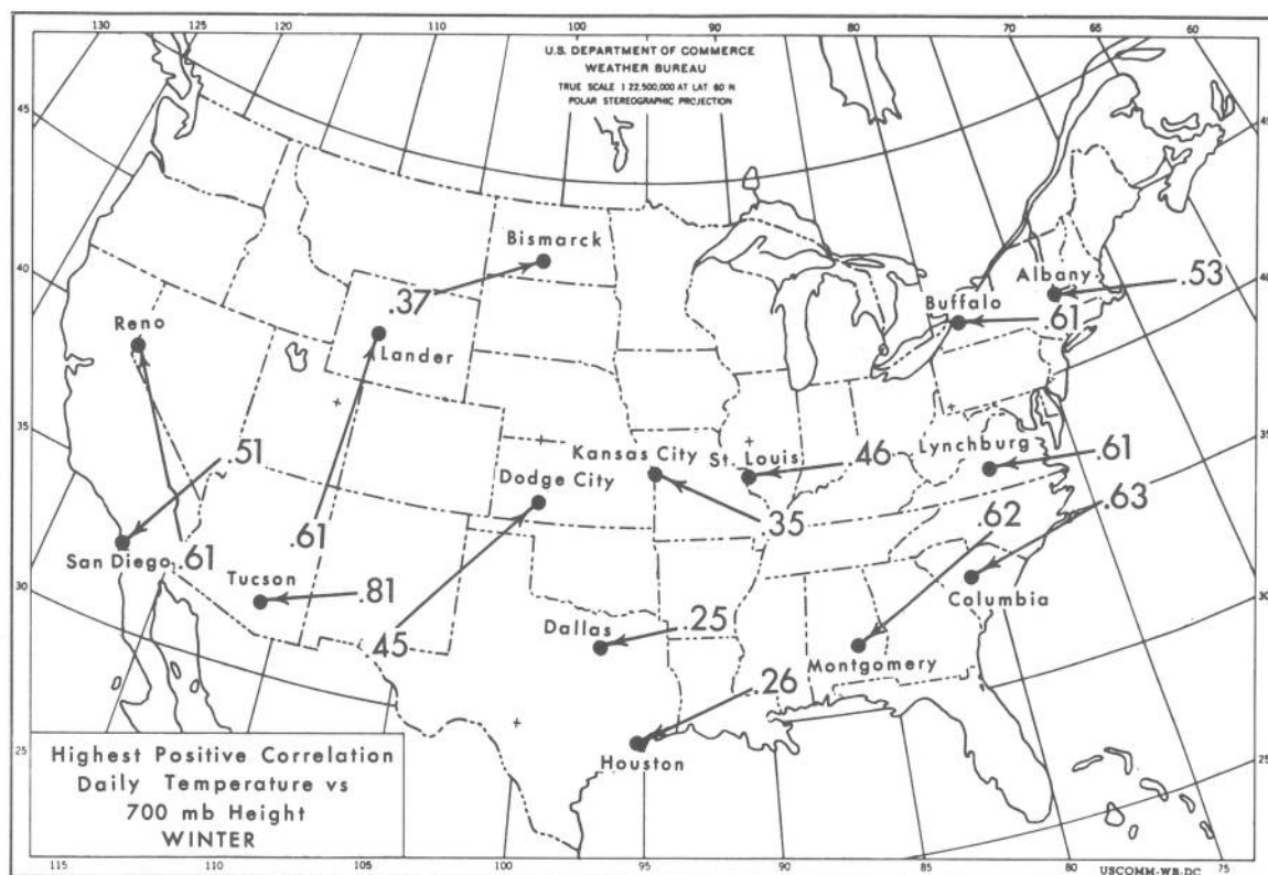
Figure 12. - Center and magnitude of maximum positive correlation between anomalies of mean daily temperature at the cities indicated and 700-mb. height on the same day for 140 winter cases.
