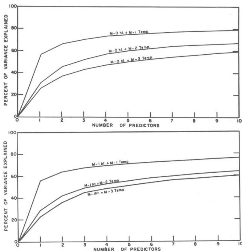
Figure 8. - Percent of variance of daily temperature anomaly in winter on M-0 day explained by the number of 700-mb. height and surface temperature predictors given along the abscissa. The results are averaged over 15 cities and are shown separately for anomalies of M-1, M-2, and M-3 temperature in conjunction with M-0 heights (above) and M-1 heights (below).
