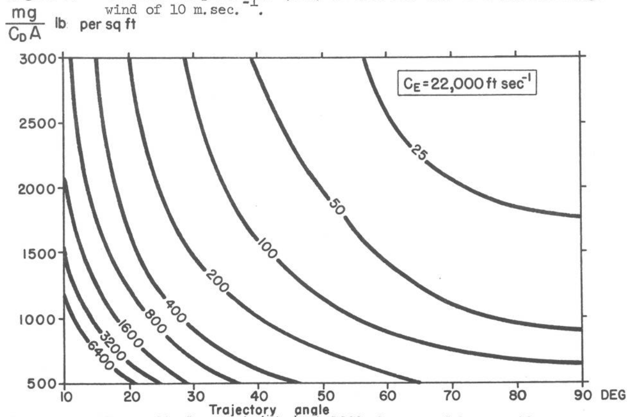
Figure 3. - Range displacement (ft.) at 1000 mb. caused by a uniform range-wind of 10 m. sec. -1 throughout the atmosphere. Re-entry speed 22,000 ft. sec. -1 .
