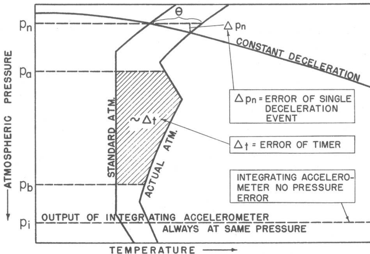
Figure 4. - Illustrating effects of non-standard atmosphere on inertial altimetry components.
