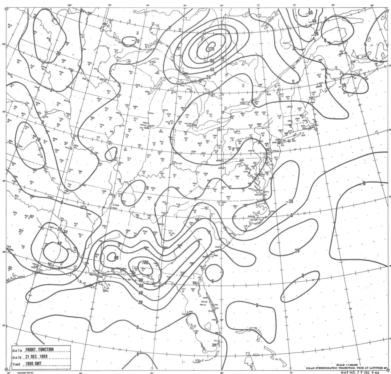
Figure 13.--The field of frontogenetical function for 1900 GMT 21 December 1969. Values have the same units as in Figure 9.
