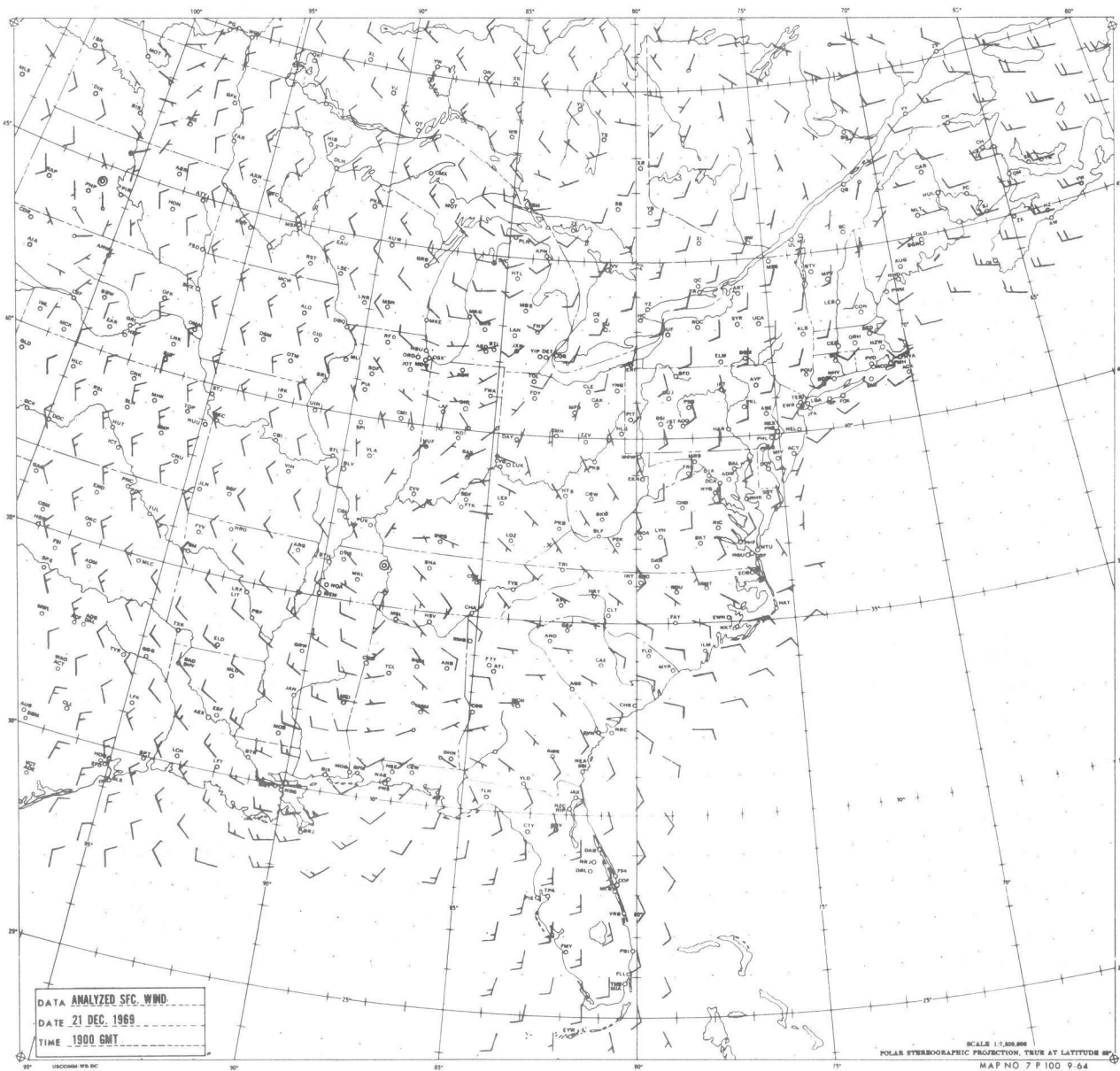
Figure 2.--The analyzed surface winds for 1900 GMT 21 December 1969, plotted at gridpoints. Symbols have their customary meaning: two concentric circles indicate calm, a shaft with no barbs indicates a speed of 1 to 2 knots, a half barb indicates a speed of 3 to 7 knots, a full barb indicates a speed of 8 to 12 knots, a full and half barb combination indicates a speed of 13 to 17 knots, etc.
