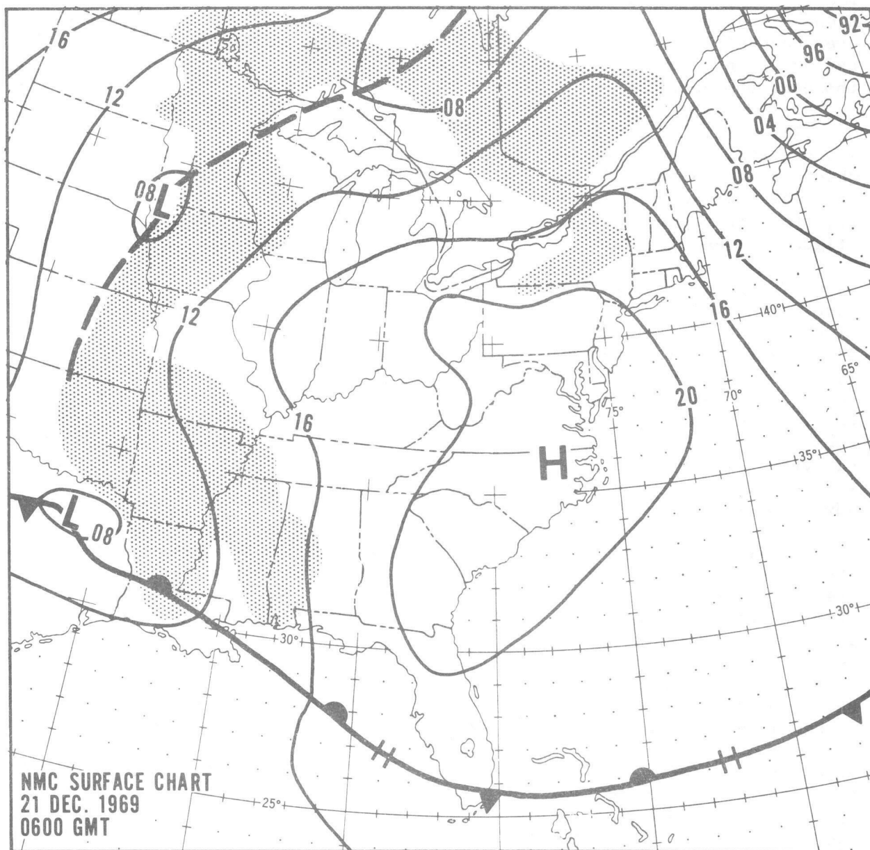
Figure 5.--The NMC sea level pressure and frontal analysis for 0600 GMT 21 December 1969.
