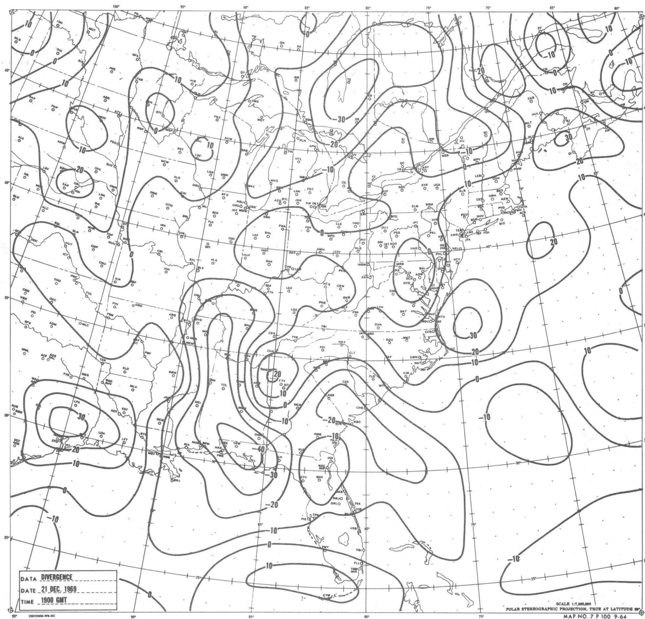
Figure 11.--The field of surface divergence for 1900 GMT 21 December 1969. Values have the same units as in Figure 7.
