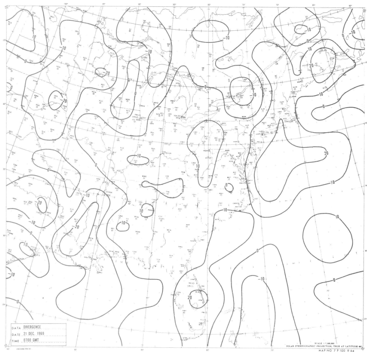
Figure 7.--The field of surface divergence for 0700 GMT 21 December 1969. Values are in units 10^{-6} \text{ sec}^{-1} . Negative values indicate convergence.
