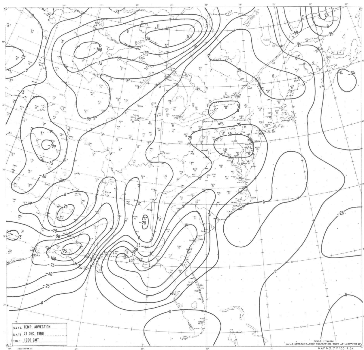
Figure 14.--The field of temperature advection for 1900 GMT 21 December 1969. Values have the same units as in Figure 10.
