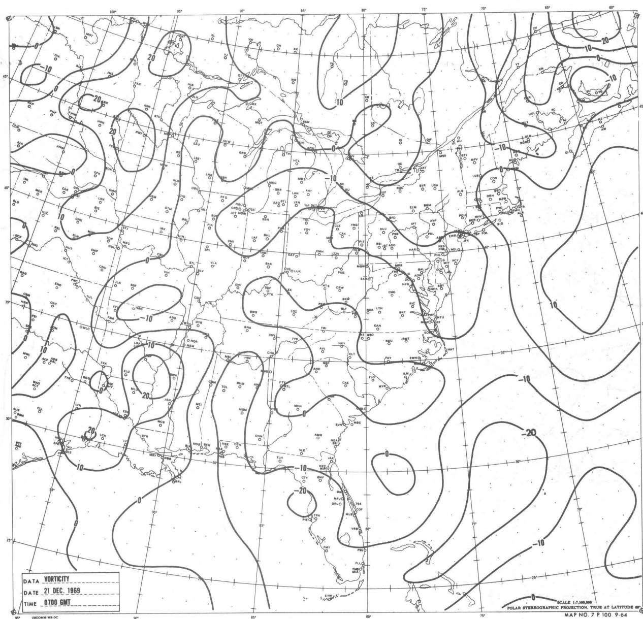
Figure 8.--The field of surface vorticity for 0700 GMT 21 December 1969. Values are in units 10^{-6} \text{ sec}^{-1} . Positive values indicate cyclonic vorticity.
