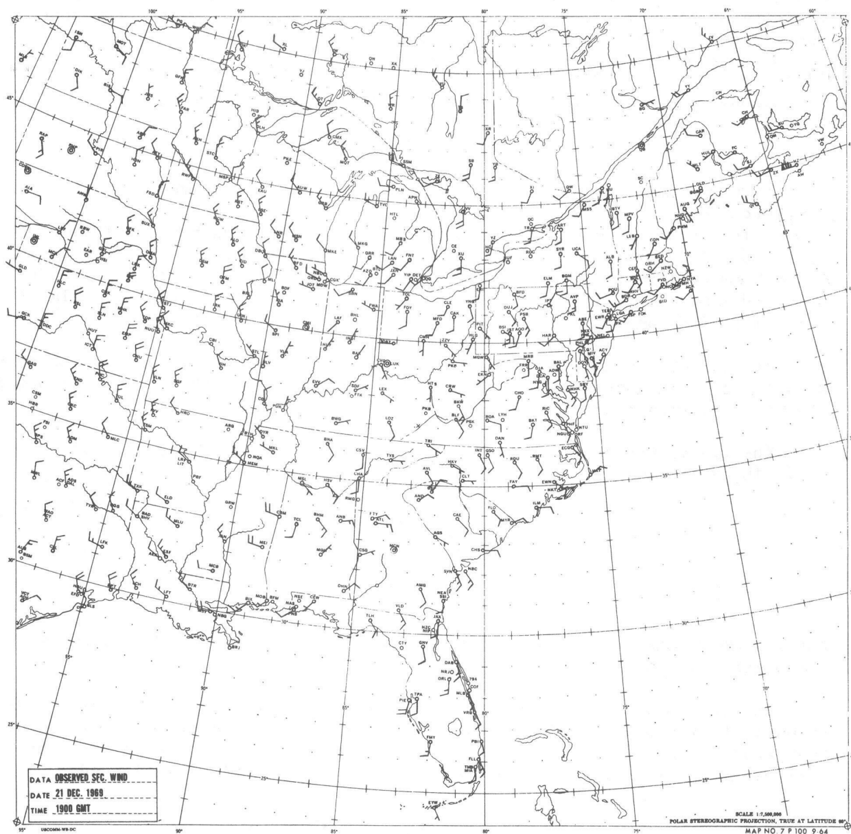
Figure 3.--The observed surface winds for 1900 GMT 21 December 1969, plotted at stations. Symbols have the same meaning as in Figure 2.
