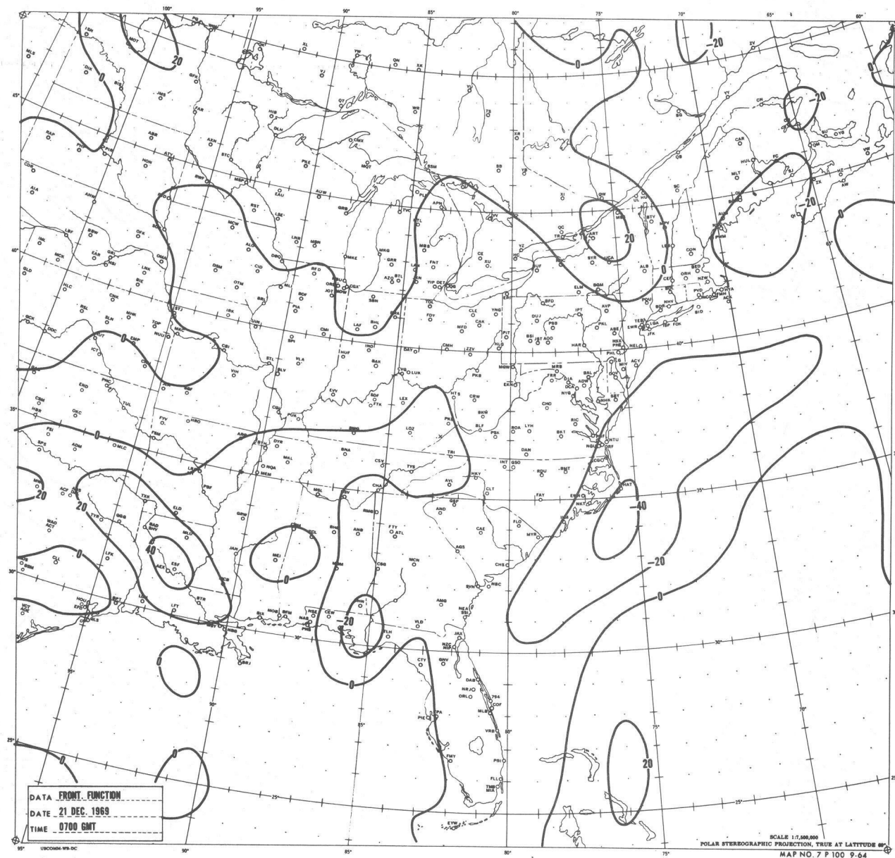
Figure 9.--The field of frontogenetical function for 0700 GMT 21 December 1969. Values are in units 10^{-11} \text{ deg.C(m.sec)}^{-1} .
