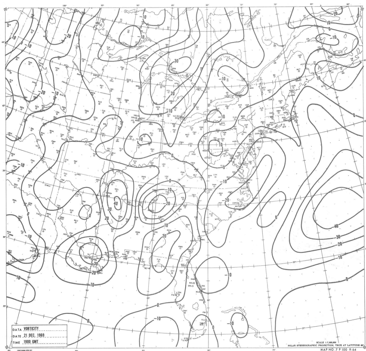
Figure 12.--The field of surface vorticity for 1900 GMT 21 December 1969. Values have the same units as in Figure 8.
