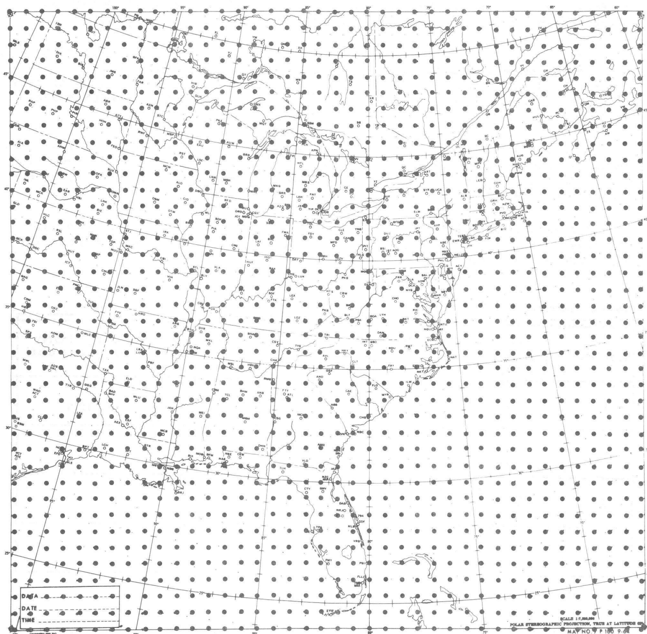
Figure 1.--The analysis and computational area, and 39 x 40 grid. The grid-length is the same as that used in SAM.
