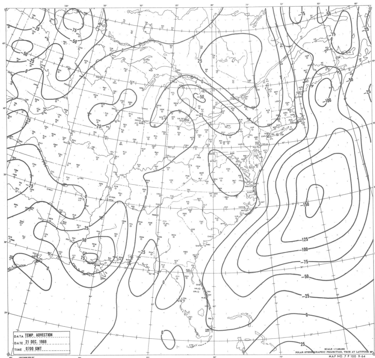
Figure 10.--The field of temperature advection for 0700 GMT 21 December 1969. Values are in units 10^{-2} \text{ deg.F}(\text{hr.})^{-1} .
