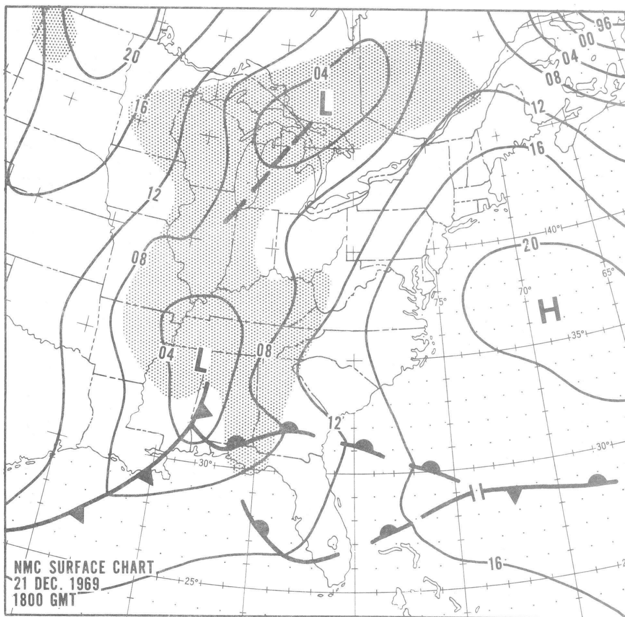
Figure 6.--The NMC sea level pressure and frontal analysis for 1800 GMT 21 December 1969.
