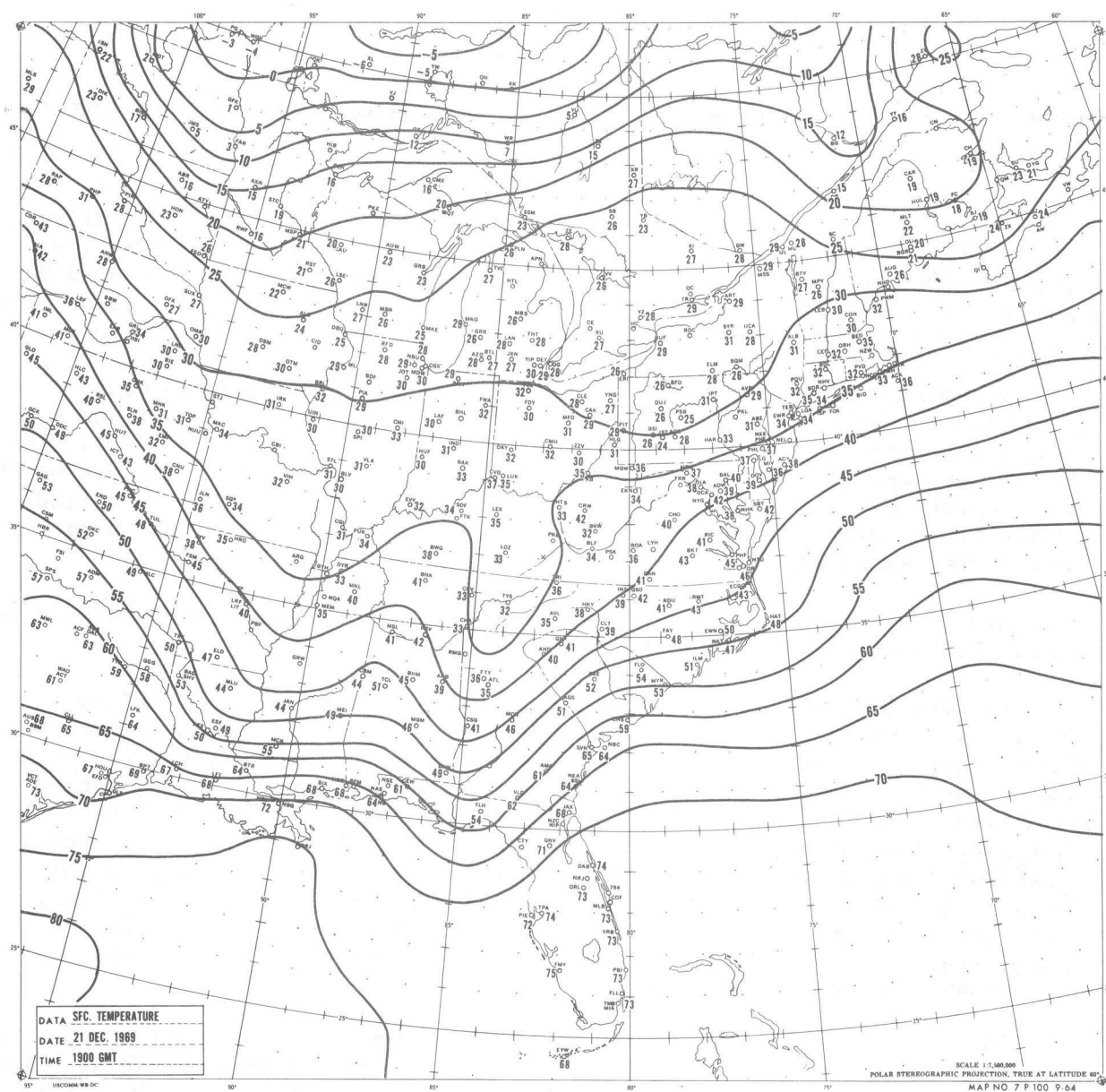
Figure 4.--The observed surface temperature and analyzed isotherms for 1900 GMT 21 December 1969. Temperatures are given in degrees Fahrenheit.
