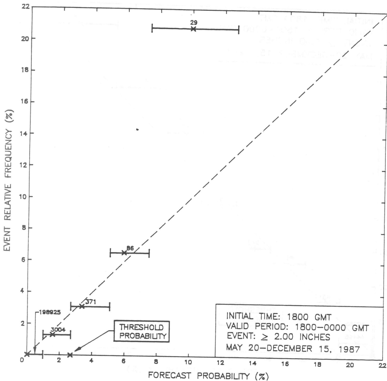
Figure 2. As in Fig. 1 except for \geq 2.00 inches. The overall sample relative frequency for the \geq 2.00 inch event was 0.07%.
