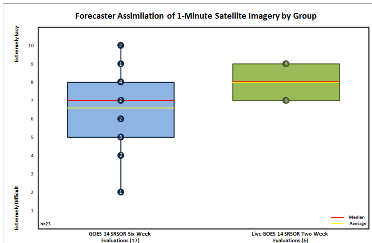
Fig. 7. As in Fig. 4 but for forecaster responses rating the ease of assimilation of 1-min satellite imagery as the warning forecaster during the 6-week evaluation and the 2-week real-time evaluations.
