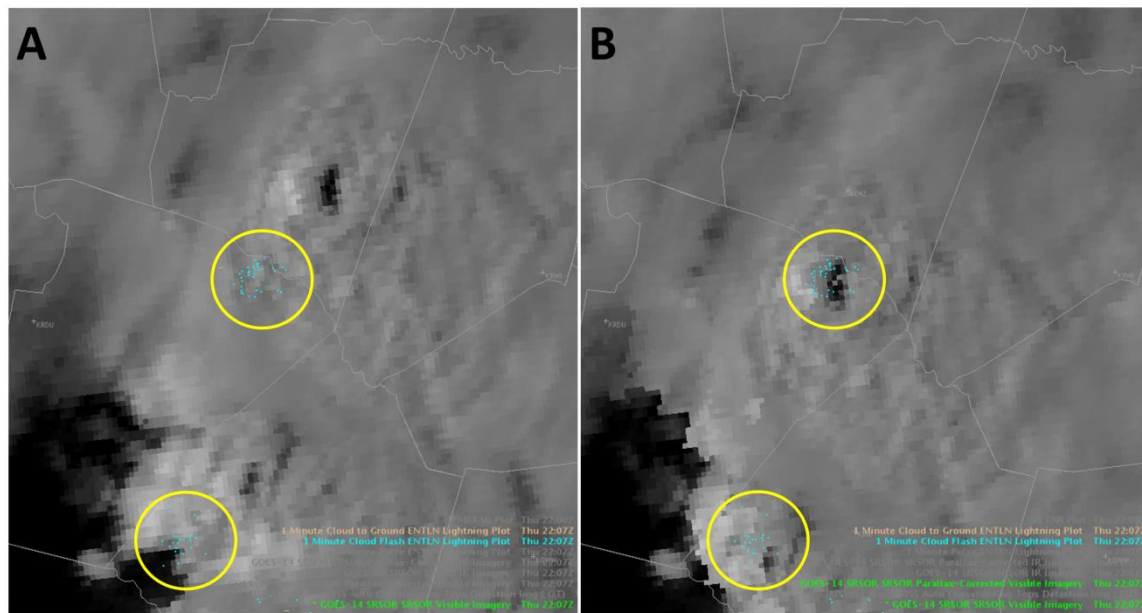
Figure 11: 2207 UTC 28 April 2016 GOES-14 1-min VIS imagery A) un-corrected and B) parallax-corrected, and ENTN cloud-to-ground (tan dash) and in-cloud (blue dot) lightning data. Yellow circles indicate core of lightning activity. Note that the parallax-corrected imagery appropriately places the overshooting top in the location of greatest total lightning activity.
