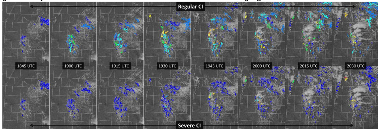
Figure 5: 1845 – 2030 UTC 28 April 2016 GOES-East VIS, regular CI (top), and severe CI (bottom).
