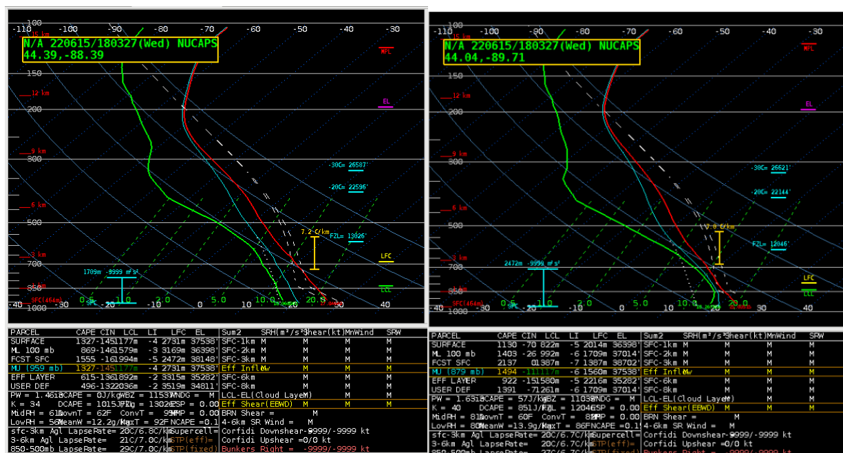
Figure 9: NUCAPS Profiles from NOAA-20 around 18Z (left) and Aqua around 19Z (right) in the Green Bay, Wisconsin CWA on 15 June 2022.
