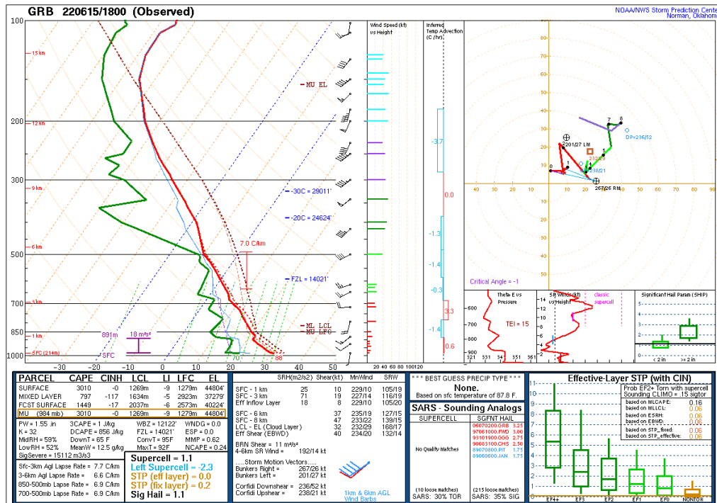
Figure 10: GRB sounding around 18Z on 15 June 2022.
