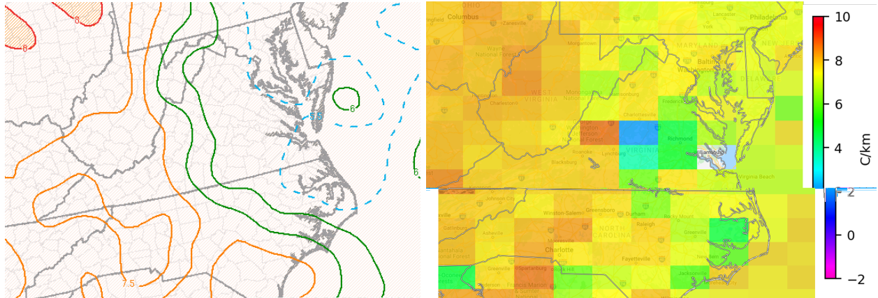
Figure 7: (Left) SPC Meso-A 700-500 mb lapse rates at 19z 6/14. (Right) NUCAPS 700-500 mb lapse rates at 1819z 6/14.
