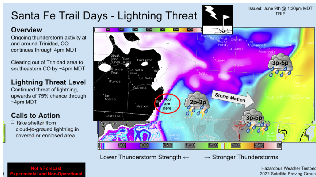
Figure 21: A public graphic featuring the PHSnMWnABI MU-CAPE field from a mock DSS event on 9 June 2022 in Colorado.
