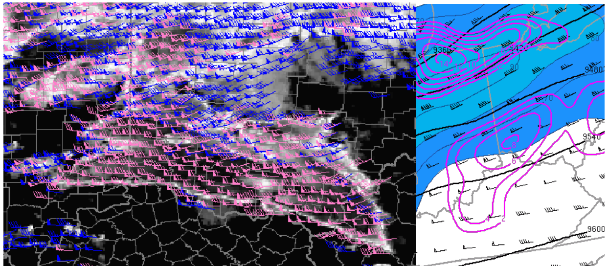
Figure 14: (Left) 400-200 mb (blue) and 200-100 mb (pink) winds from the Optical Flow Winds product on 8 June 2022 near 2100 Z. (Right) 300 mb geopotential heights (black), winds, and divergence (pink) fields from the 2100 Z SPC Mesoanalysis on 8 June 2022.
