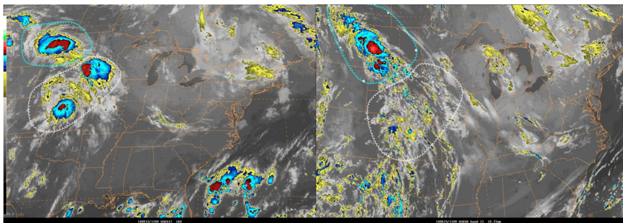
Figure 20. 20140815 1100 UTC IR imagery (left) and simulated satellite imagery (right). Three distinct MCSs were occurring in the central U.S. on this morning, but the modeled IR only forecast one.
