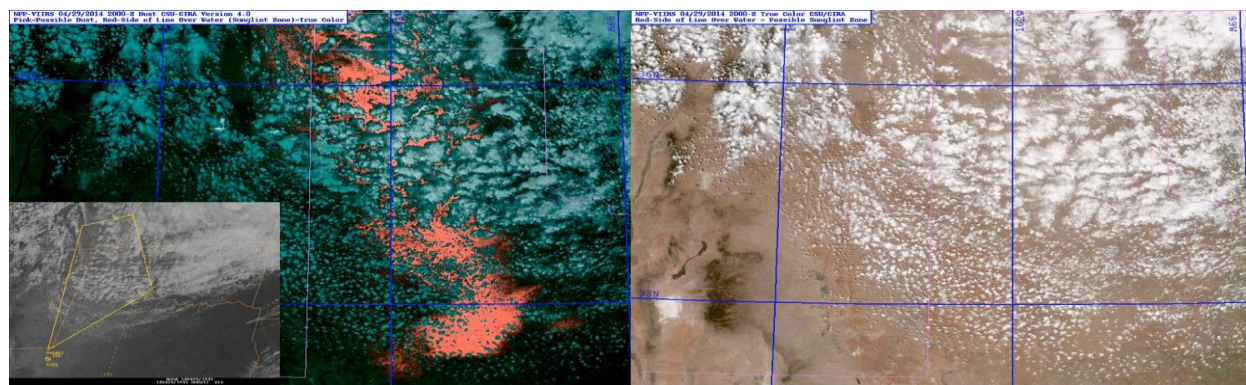
Figure 21. 20140429 2000 UTC VIIRS True Color (right) and dust enhancement (left), and the issued blowing dust SIGMET (bottom left). Dust enhancement images courtesy of Steve Miller, CIRA.
