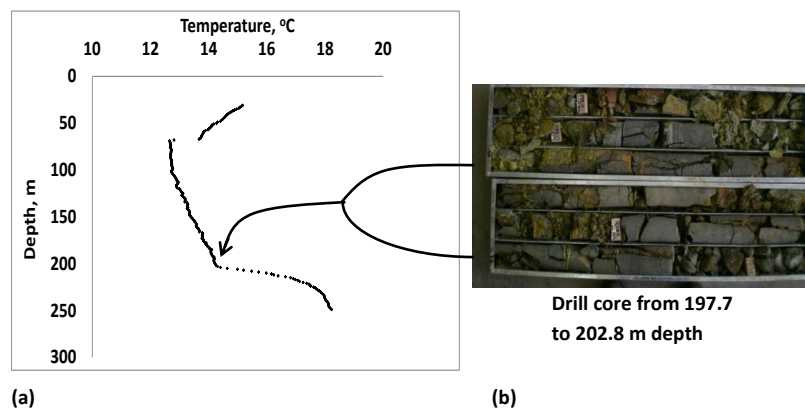
Figure 6. (a) Borehole temperature profile (Oatlands borehole) suspected to have been affected by groundwater movement at \sim 200 m. The upper discontinuity may be due to horizontal groundwater flow. (b) Broken drill core from 197.7 to 202.8 m depth. The high frequency of fractures suggests highly permeable rock and groundwater movement (Photo courtesy of Oatlands borehole, KUTh energy, Tasmania).
