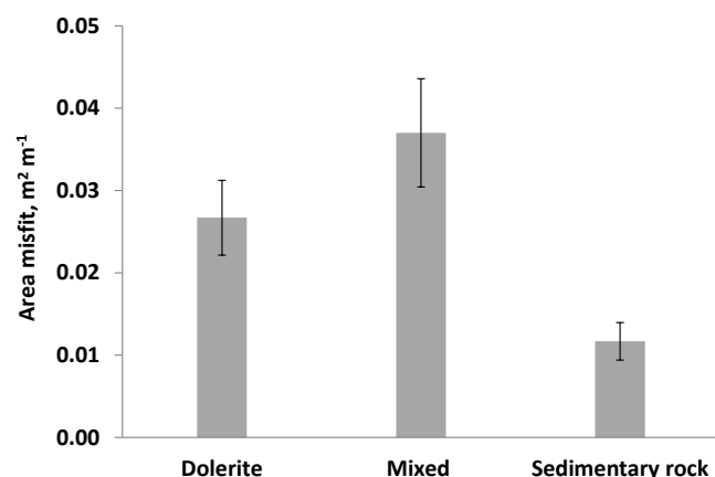
Figure 7. Relationship between area misfit and borehole sub-surface lithology. Error bars represent standard errors, with a 1\sigma confidence interval.
