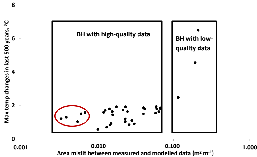
Figure 5. GTC with an area misfit between measured and modelled data.
