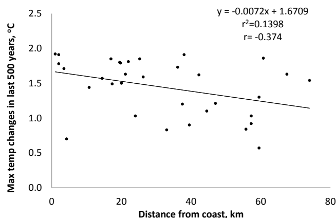
Figure 10. Correlation between the GTC and the distance of the borehole location from the coast.
