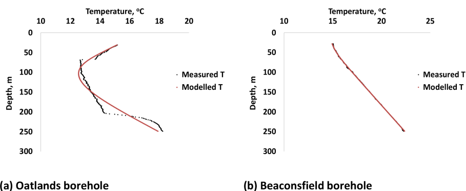
Figure 3. (a) High deviation between measured and modelled temperature–depth profile and borehole records classified as low quality. (b) Very low deviation between measured and modelled temperature–depth profile and borehole records classified as high quality.
