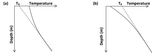
Figure 2. Schematic diagram of borehole temperature–depth profiles showing ground surface temperature (a) warming and (b) cooling. Dashed and Solid line indicates the steady-state and measured temperature respectively. T_0 represent ground temperature at steady-state condition.
