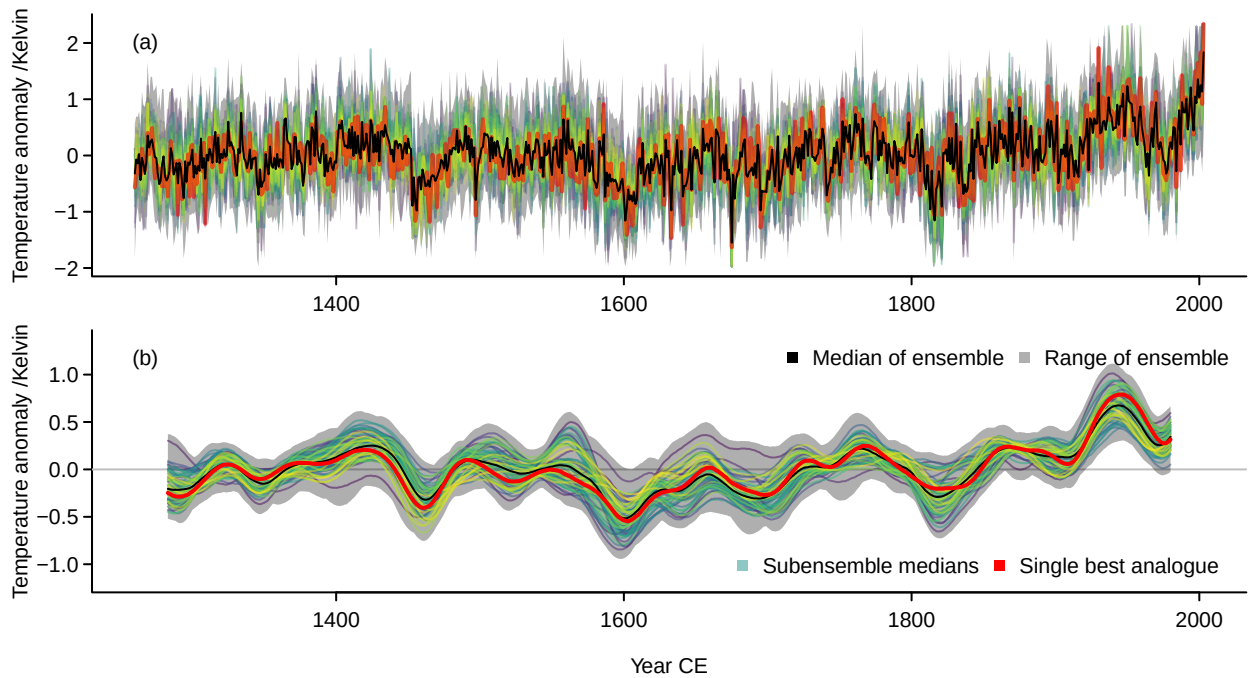
Figure 11. Comparison of local grid-point analogue data with an ensemble of regionally-representative subsampled reconstructions: (a) Interannual data from BEST. Location, station-name, and correlation over available station (b) data are at smoothed with 47-point Hamming filter. Both panels show in grey the top full range of the panels. Grey 6500 reconstructions based on 4 proxies and only half of the simulated fields, in black the median of all 6500 reconstructions, interannual and smoothed in red the single best analogue median. Red and blue, station reconstruction based on the full data and its smooth. X-axes are years CE. Y-axes Further colored lines are temperature anomalies in degree Kelvin relative to medians of the period where both datasets are available 65 subensembles using different sets of 4 proxies. Panel (b) adds a zero line as visual assistance.
