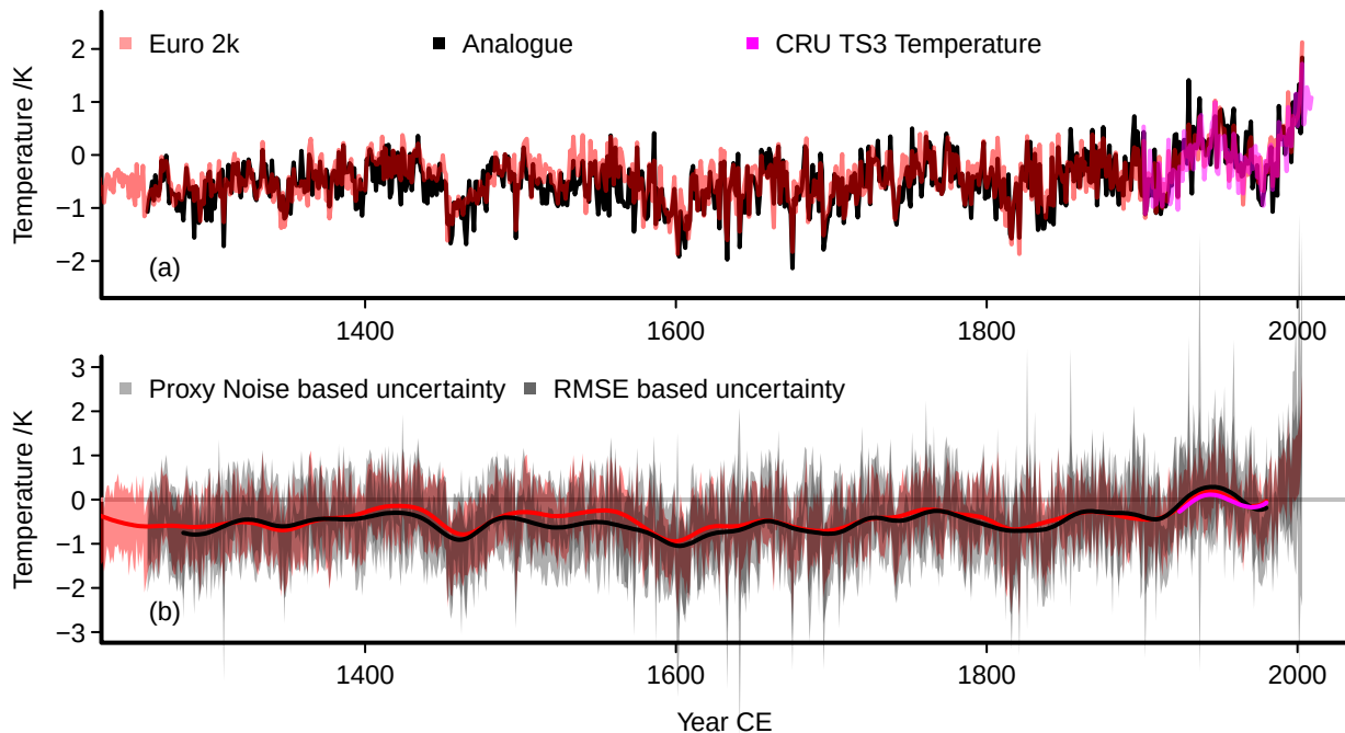
Figure A1. The best-analogue reconstruction as in Figure 2 but relative to the observational period 1901-2003 CE: (a) the interannual temperature reconstruction in black, the red line is the area mean Euro 2k-reconstruction, magenta is the observational CRU temperature adjusted to the mean of the reconstruction over its time-range. The analogue reconstruction is rescaled by the variability from one of the simulations. (b): as (a) but for 47-point Hamming filtered data; we further add the uncertainty for estimates for the interannual data: red is the unsmoothed Euro 2k-uncertainty, the lighter grey envelope is a 2 standard-deviation uncertainty based on the correlation between the the proxies and the observations at the proxy locations, the darker grey envelope is a 2 standard-deviation uncertainty based on a MSE-estimate. Panel (b) adds a zero line as visual assistance.
