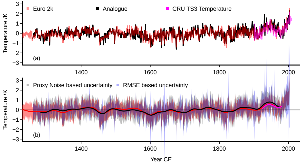
Figure 2. Summary of the The best-analogue reconstruction relative to its full period mean : (a) the interannual rescaled temperature reconstruction in black and an 50% uncertainty in grey based on the correlation between the the proxies and the observations at the proxy locations ; the red line is the area mean Euro 2k-reconstruction; magenta is the observational CRU temperature adjusted to the mean of the reconstruction over its time-range. The analogue reconstruction is rescaled by the variability from one of the simulations. (b): as (a) but for 47-point Hamming filtered data; we further add the uncertainty for estimates for the interannual data : red shading is the unsmoothed Euro 2k-uncertainty; the narrower additional grey envelope is a 50%-2 standard-deviation uncertainty based on an MSE-estimate. (c): Difference between the Euro 2k and the analogue reconstruction and its smooth. (d): Ratio-correlation between the standard-deviations of proxies and the analogue values observations at the closest grid-points to the proxy values. (e): Mean squared-error between analogue grid-point values and locations , the proxies blue envelope is a 2 standard-deviation uncertainty based on a MSE-estimate. Panel (b) adds a zero line as visual assistance.
