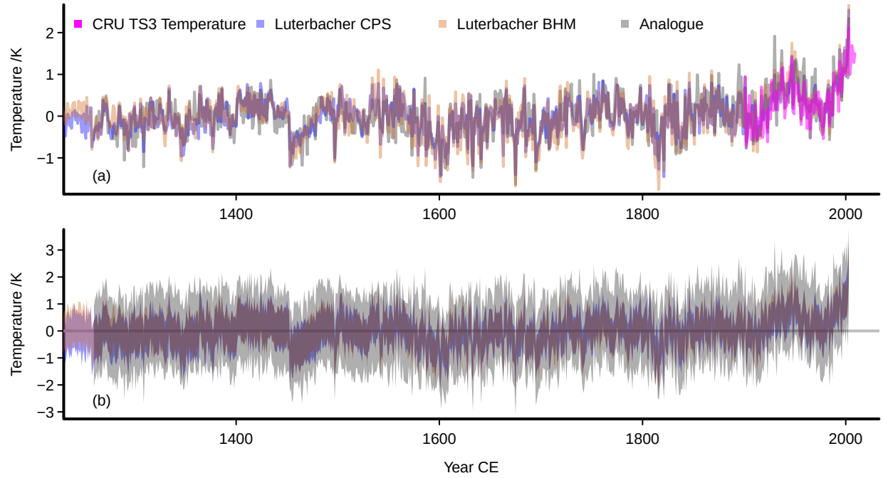
Figure A3. Comparison of the reconstructions of Luterbacher et al. (2016) to the best-analogue reconstruction (see also Figure 2): (a) the interannual single best analogue temperature reconstruction in grey; the blue is the composite plus scale (CPS) reconstruction of Luterbacher et al. (2016) and the brown line is the area mean of their Bayesian Hierarchical Modelling reconstruction; magenta is the observational CRU temperature adjusted to the mean of the analogue reconstruction over its time-range. The analogue reconstruction is rescaled by the variability from one of the simulations. (b): as (a) but for the 95% uncertainties of the reconstructed datasets. Differences between the Luterbacher CPS and the Euro 2k mean reconstructions are smaller than 0.005K. Panel (b) adds a zero line as visual assistance.
