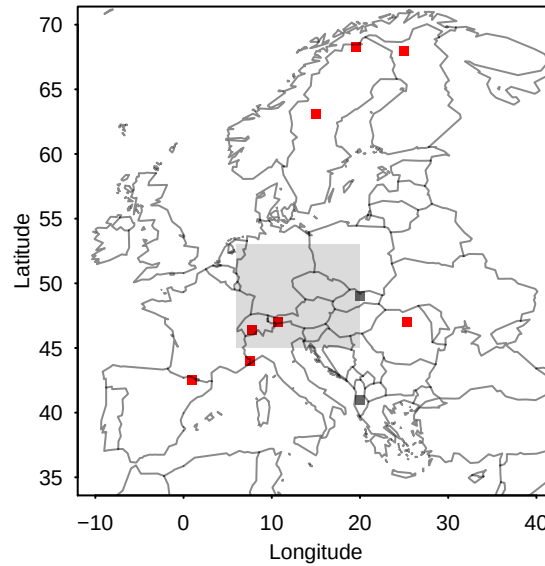
Figure 1. Reconstruction domain and locations of the included proxies. Red squares show the proxies included in our search, grey squares show the locations from the original Euro 2k setup, which we exclude. The grey shaded box shows the original domain of Dobrovolný et al. (2010).
