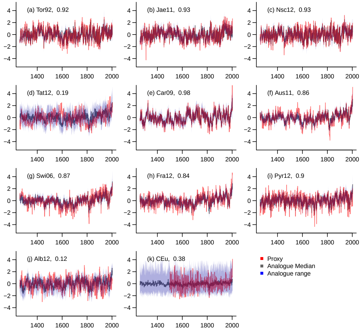
Figure 6. Analogue reconstruction values at the locations of the Euro 2k-proxies. Shown are the normalized proxies in red, the median of 39 analogue values in black and the full range of the 39 local analogues in blue. X-axes are years CE. Correlations between the local reconstruction median and the proxy series are given as numbers next to the proxy IDs in each panel.
