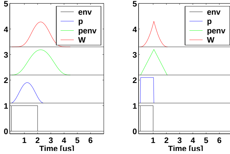
Figure 7: The transmitter envelope (env), filter impulse response (p), effective pulse form (penv) and the range weighting function (W) using a realistic impulse response (left) and a box-car impulse response (right)
