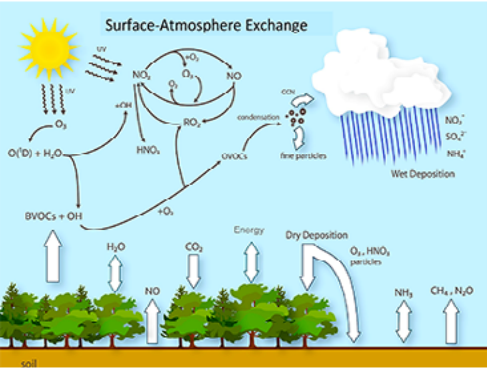
The complex chemistry and dynamics of the surface atmospheric exchange are depicted in this diagram. Solar radiation (UV) initiates a number of chemical processes.
