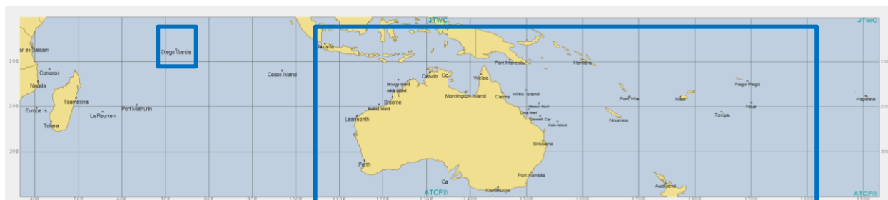
Figure 58: In the southern hemisphere, JTWC warning frequency increases from 2 per day to 4 per day within the blue boxes for DOD, American asset, and humanitarian reasons. JTWC always provides 4 warnings per day for storms in the northern Hemisphere.
