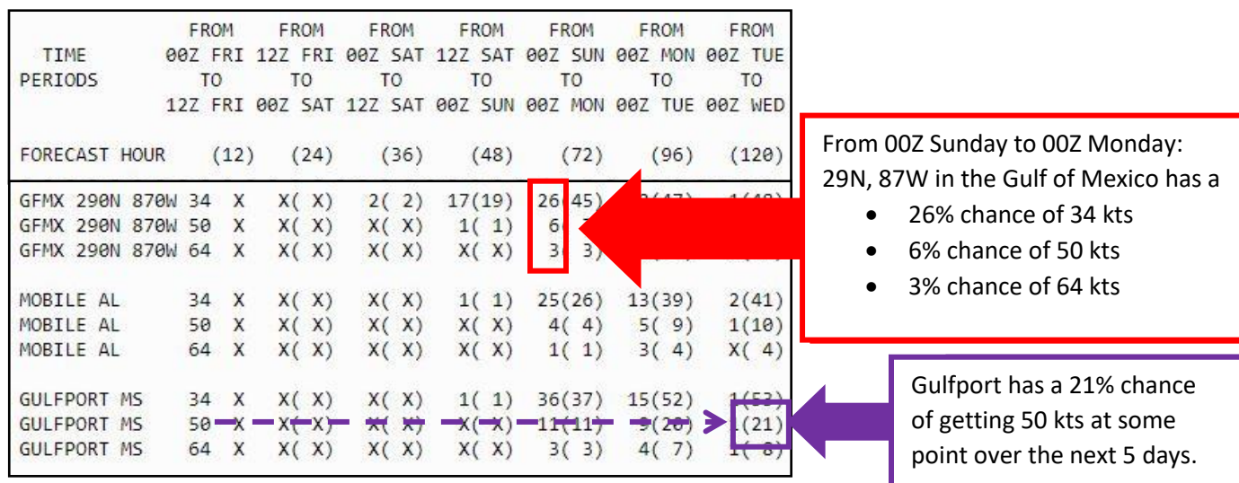
Figure 39: Annotated Tropical Cyclone Surface Wind Probabilities (PWS).
