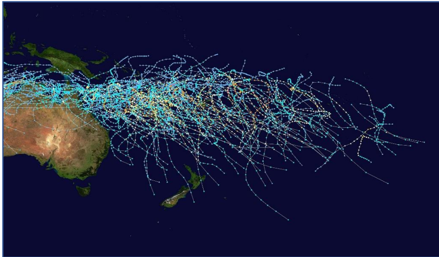
Figure 28: Southwest Pacific tropical cyclone tracks from 1980- 2005.
