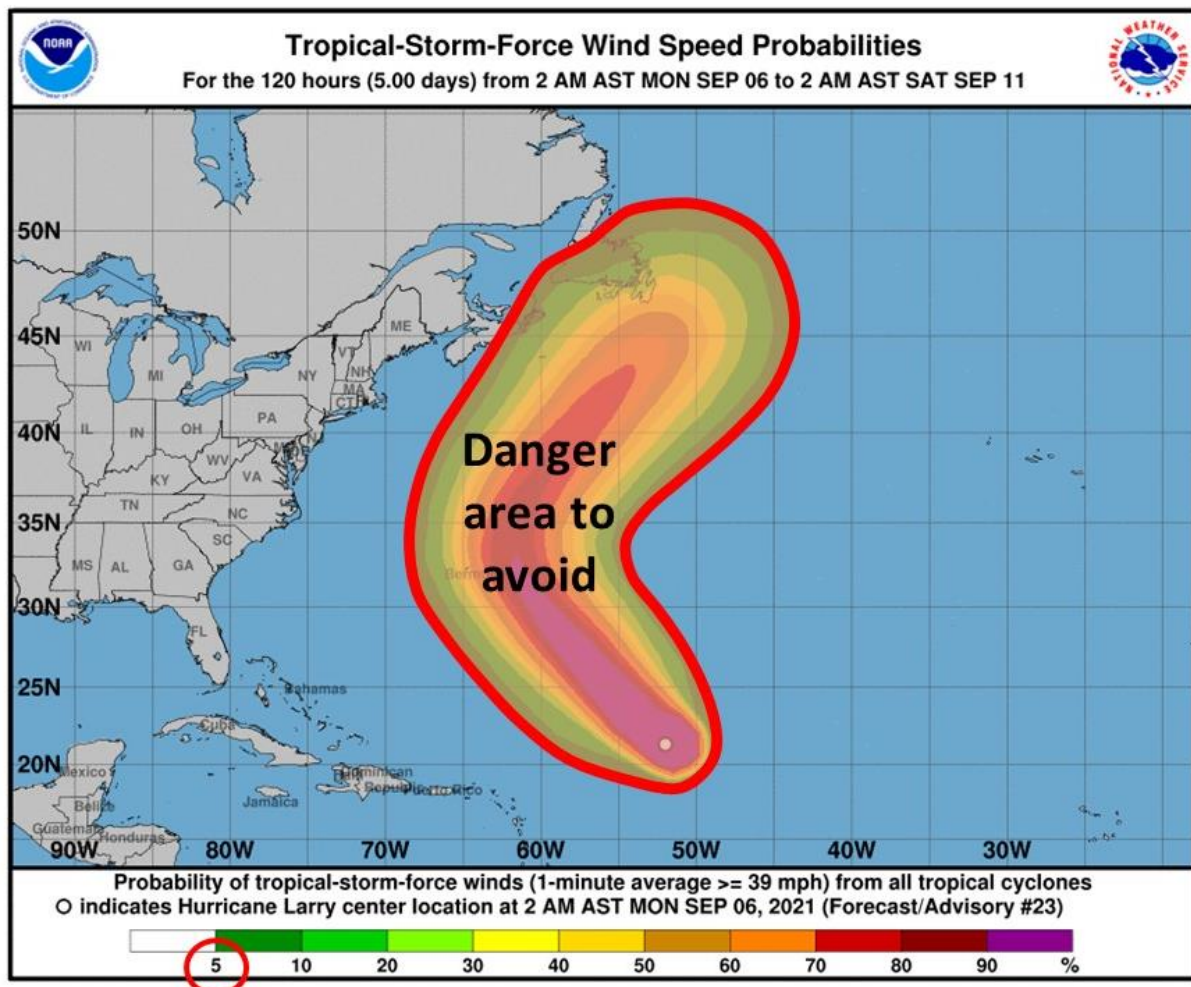
Figure 64: Using the Tropical-Storm-Force Wind Speed Probability graphic as a ship routing tool.
