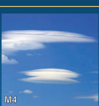
M4 Altostratus Lenticularis: Lens or almond shaped, often formed by air moving over hills or mountains.
