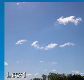
L1 Cumulus: Thin and ragged with continuously changing edges; forms during fair weather by daytime heating.
