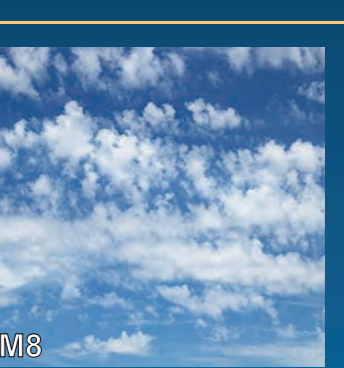
M8 Altostratus: Small towers, which can be similar to small Cumulus with wispy trails of virga.
