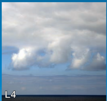
L4 Stratocumulus: Spread out Cumulus when vertical development stabilizes; sometimes can occur along with Cumulus .
