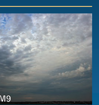
M9 Altostratus: Chaotic sky with multiple layers and kinds of Altostratus at several altitudes.
